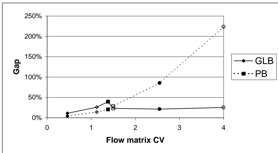
Figure 3. Gaps for bounds on grid-based QAPs
