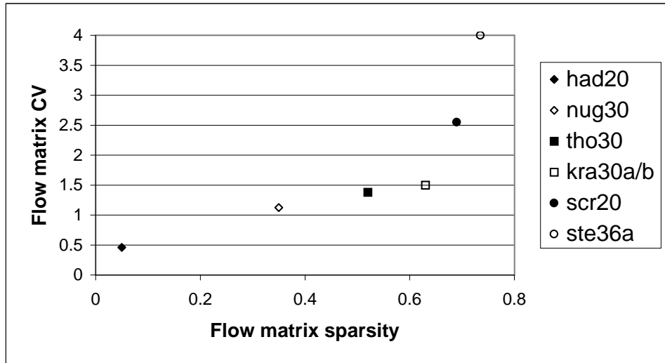
Figure 2. Characteristics of flow matrices of grid-based QAPs
