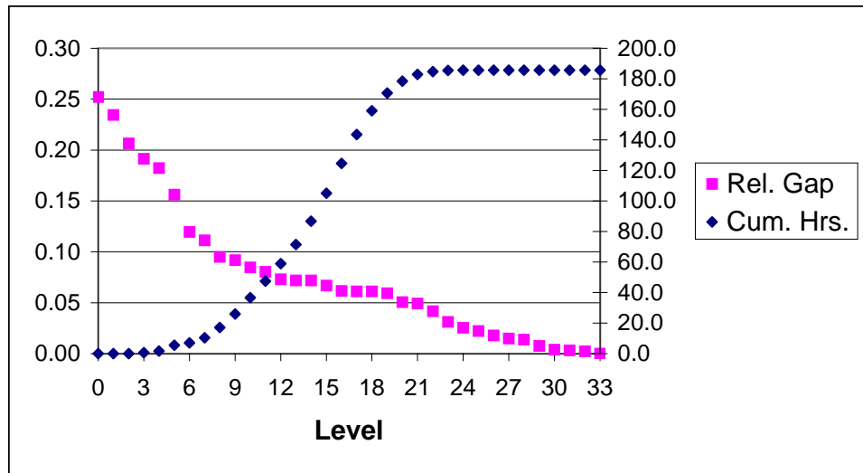
Figure 5. Relative gap and cumulative time in solution of ste36a
