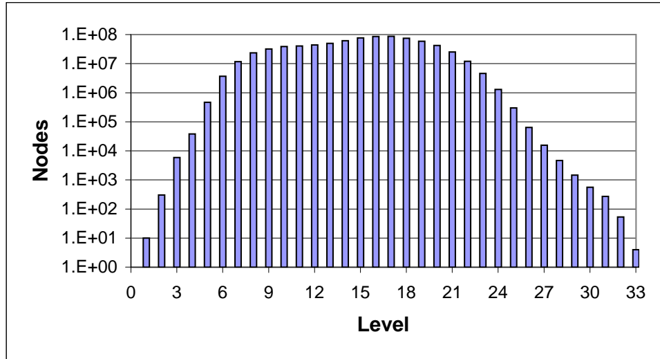
Figure 4. Distribution of nodes in solution of ste36a
