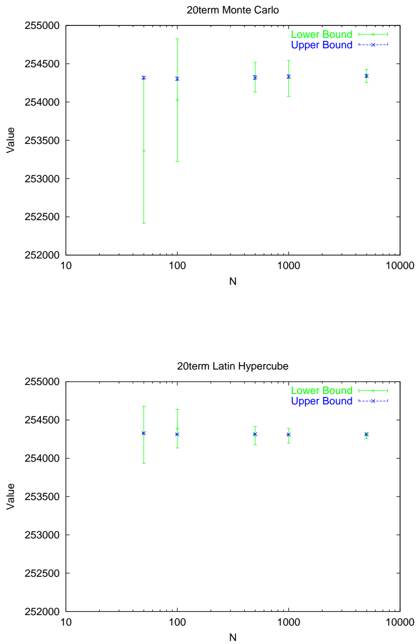
Fig. 1. 20term: Means and 95% Confidence Intervals for Optimal Value Bound Estimates
