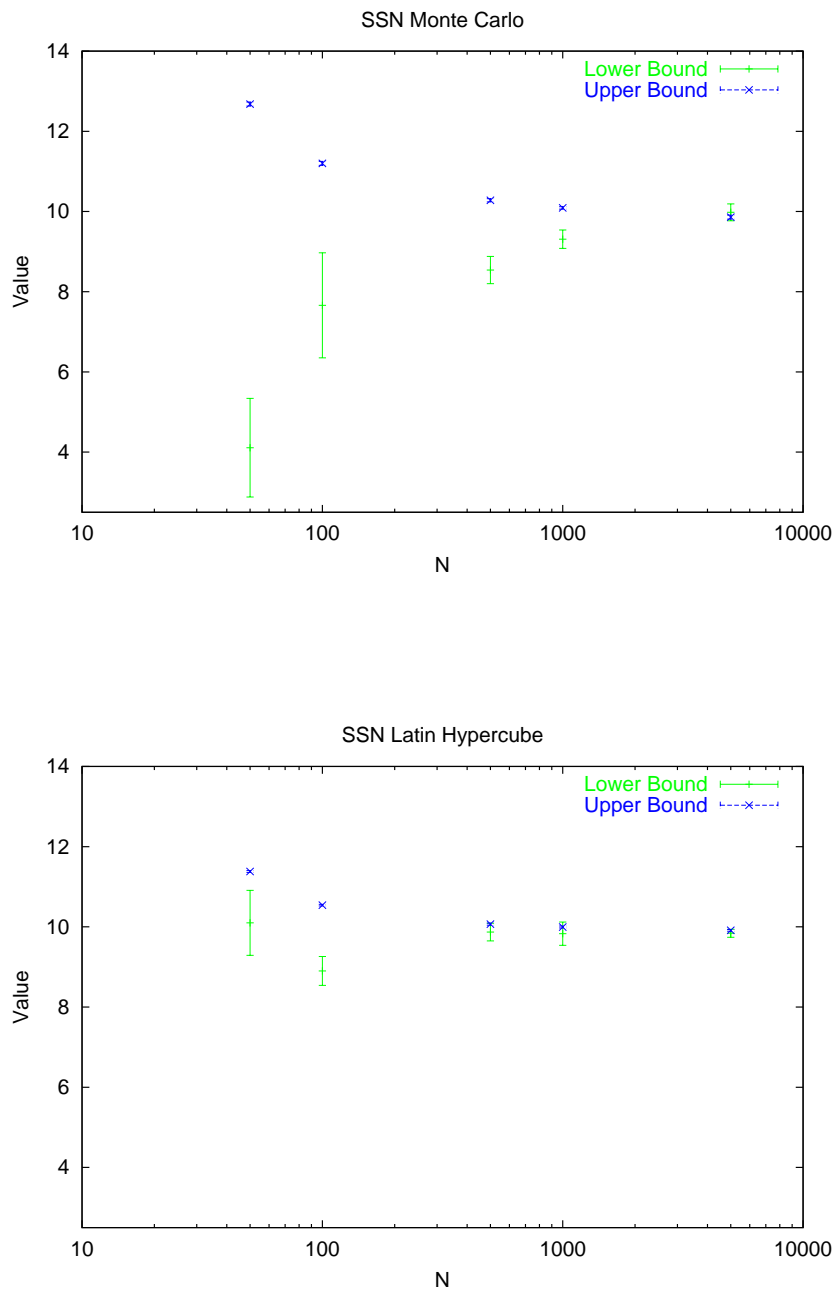
Fig. 4. SSN: Means and 95% Confidence Intervals for Optimal Value Bound Estimates
