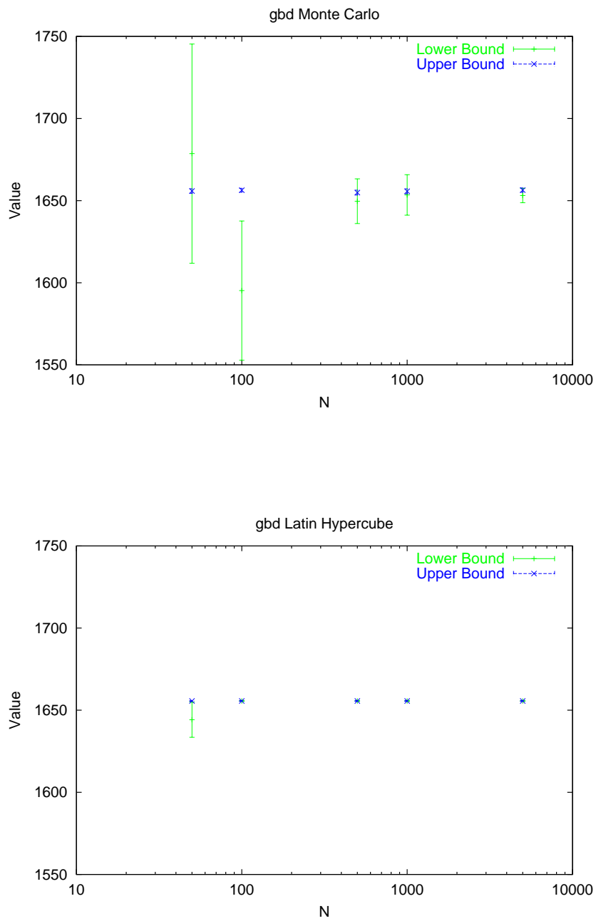
Fig. 2. gbd: Means and 95% Confidence Intervals for Optimal Value Bound Estimates
