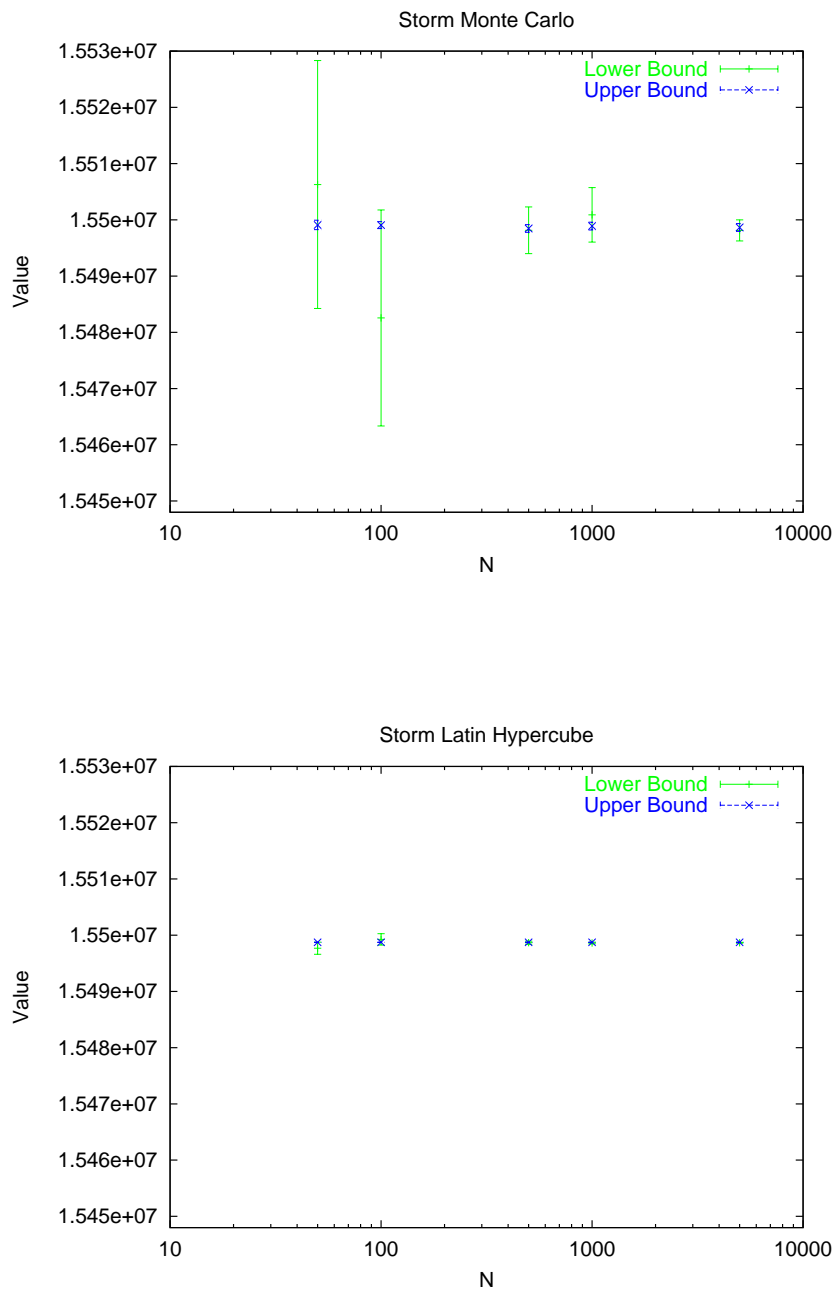
Fig. 5. storm: Means and 95% Confidence Intervals for Optimal Value Bound Estimates
