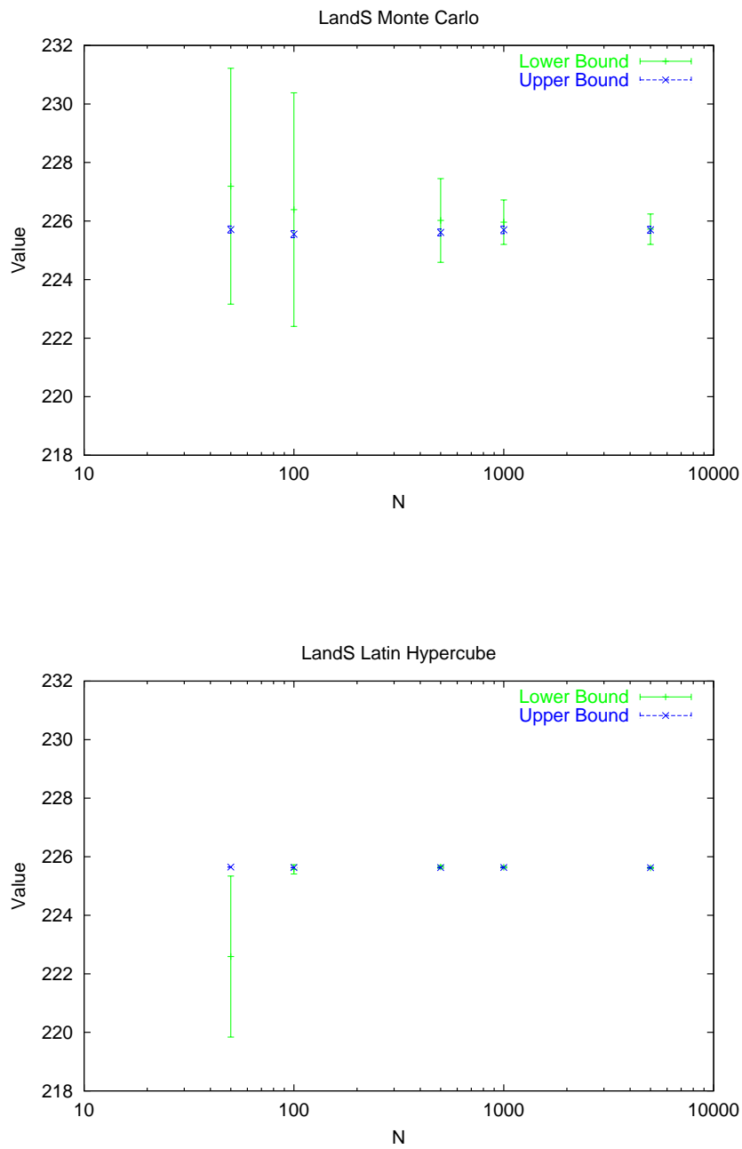
Fig. 3. LandS: Means and 95% Confidence Intervals for Optimal Value Bound Estimates
