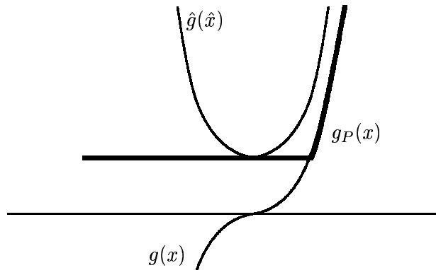
Figure 2: The surrogate g_P = \hat{g} \circ P is bounded below despite the fact that the fine model g is unbounded.
