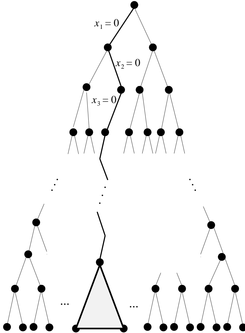
Figure 2: The figure uses the tree metaphor for our solution strategy. By solving ( SDP ) and determining members of the optimal active set, only the small shaded set of QP-subproblems need to be initially considered. Here the bold lines illustrate where activity decisions have been made within the tree.
