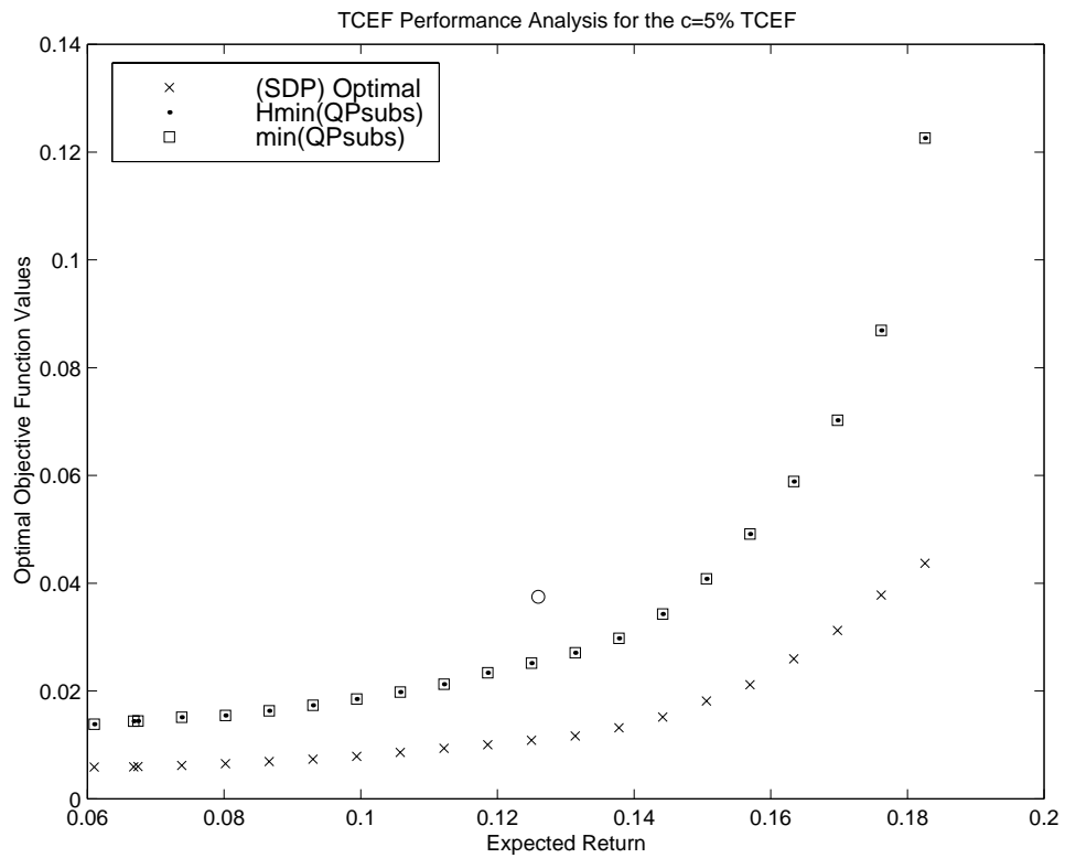
Figure 8: The circle again locates the initial portfolio. This figure presents information regarding the performance of our solution strategy.
