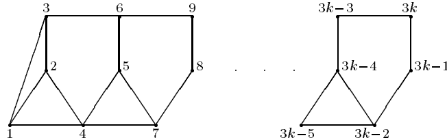
Figure 7: The graph G_k .
