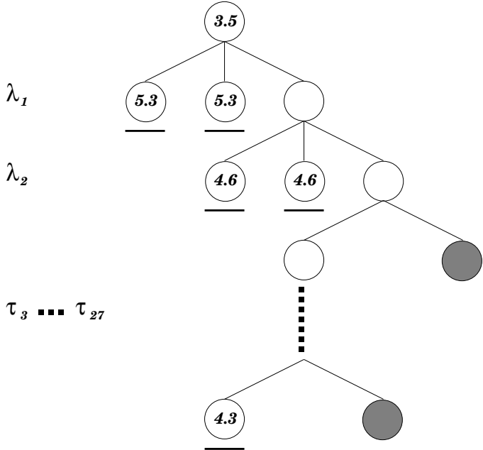
Figure 1: Branch-and-bound tree for the numerical example
