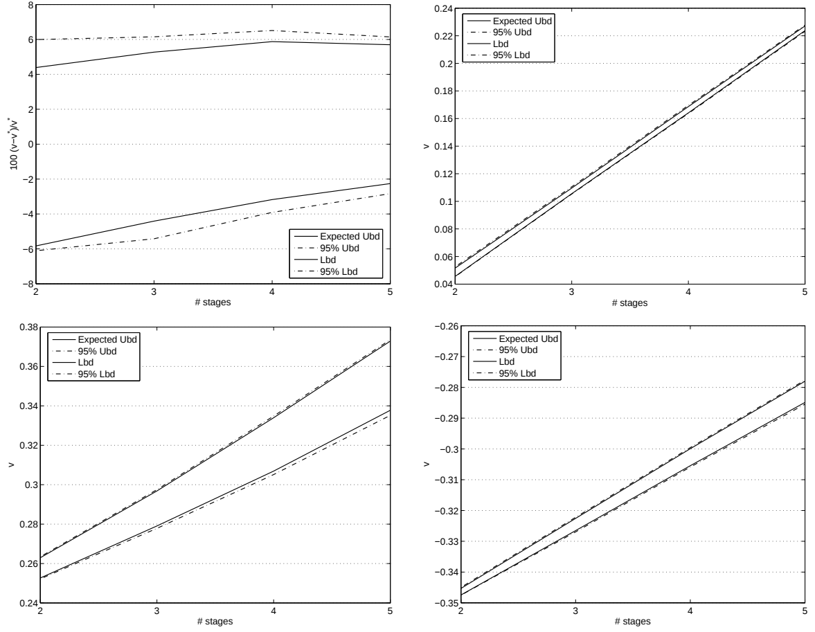
Figure 4: Objective function values for varying number of stages. Upper left: Scaled logarithmic utility function. Upper right: Logarithmic utility function with transaction costs. Lower left: Piecewise linear utility function. Lower right: Exponential utility function.
