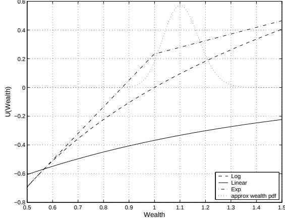
Figure 1: Objective functions used in numerical results.
