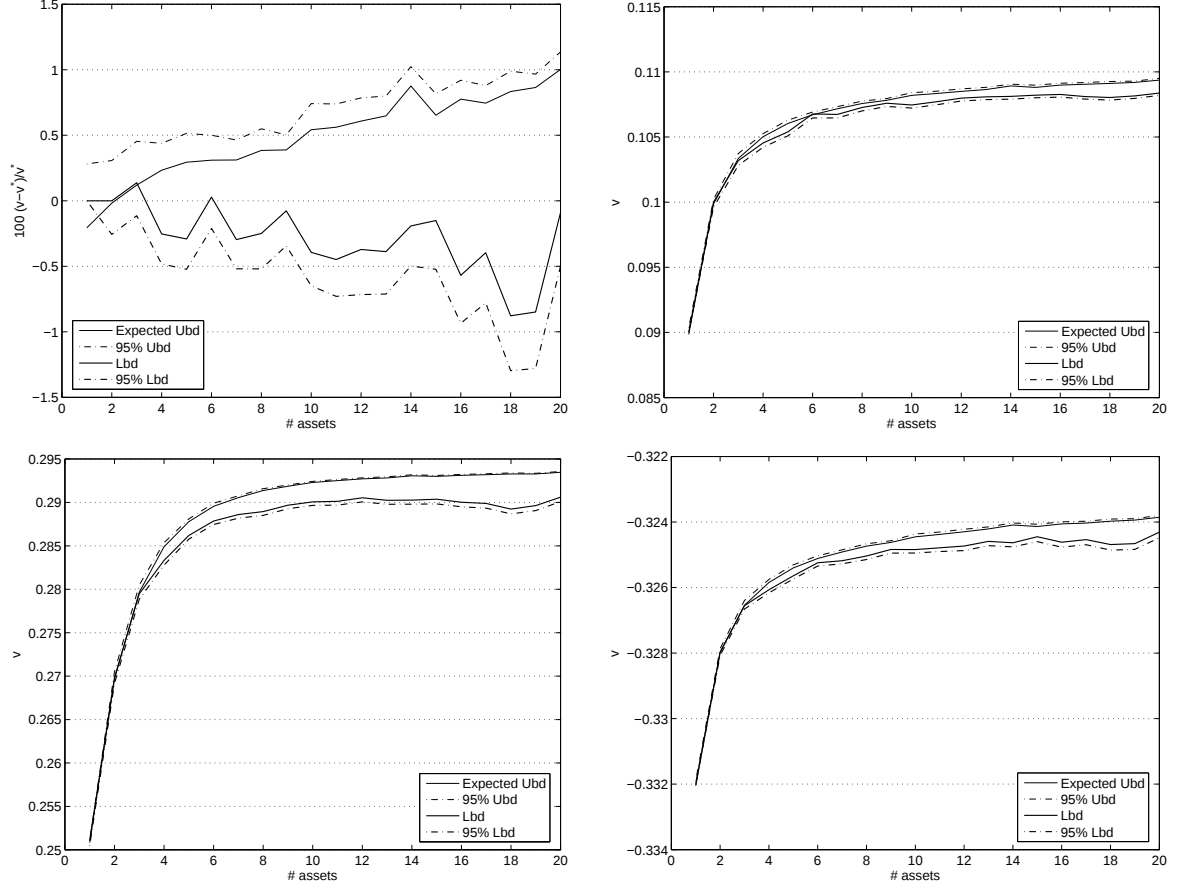
Figure 8: Objective function values for varying number of assets. Upper left: Scaled logarithmic utility function. Upper right: Logarithmic utility function with transaction costs. Lower left: Piecewise linear utility function. Lower right: Exponential utility function.
