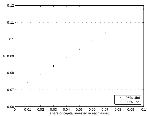
Figure 11: The quality of different first stage decisions.
