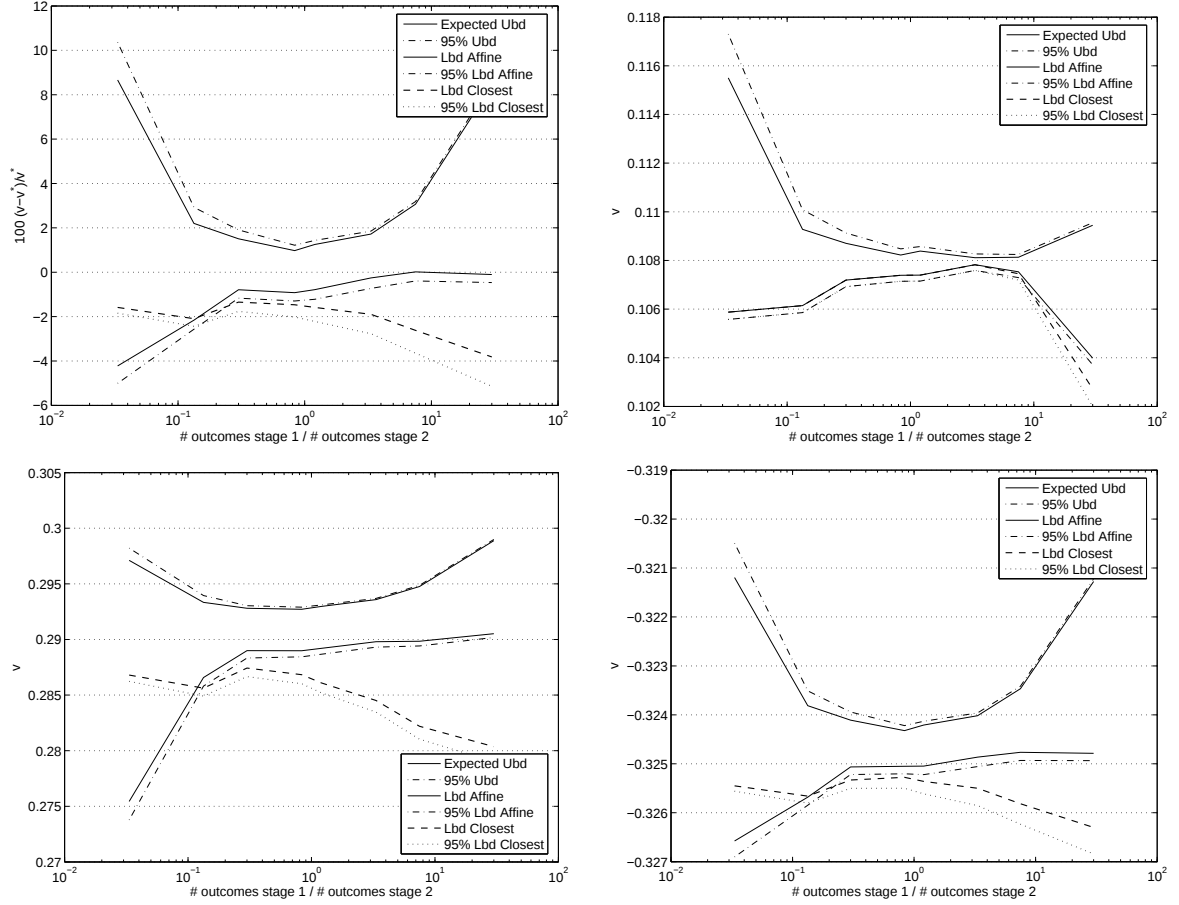
Figure 2: Objective function values for different tree structures and heuristics for determining Lbd. Upper left: Scaled logarithmic utility function. Upper right: Logarithmic utility function with transaction costs. Lower left: Piecewise linear utility function. Lower right: Exponential utility function.
