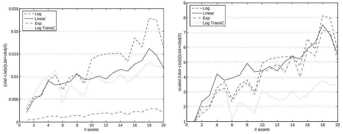
Figure 9: Left: Gap between 95% upper bound and 95% lower bound for varying number of assets. Right: Same as left but scaled.
