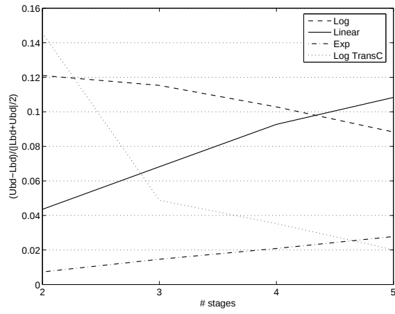
Figure 5: Gap between 95% upper bound and 95% lower bound for varying number of stages.
