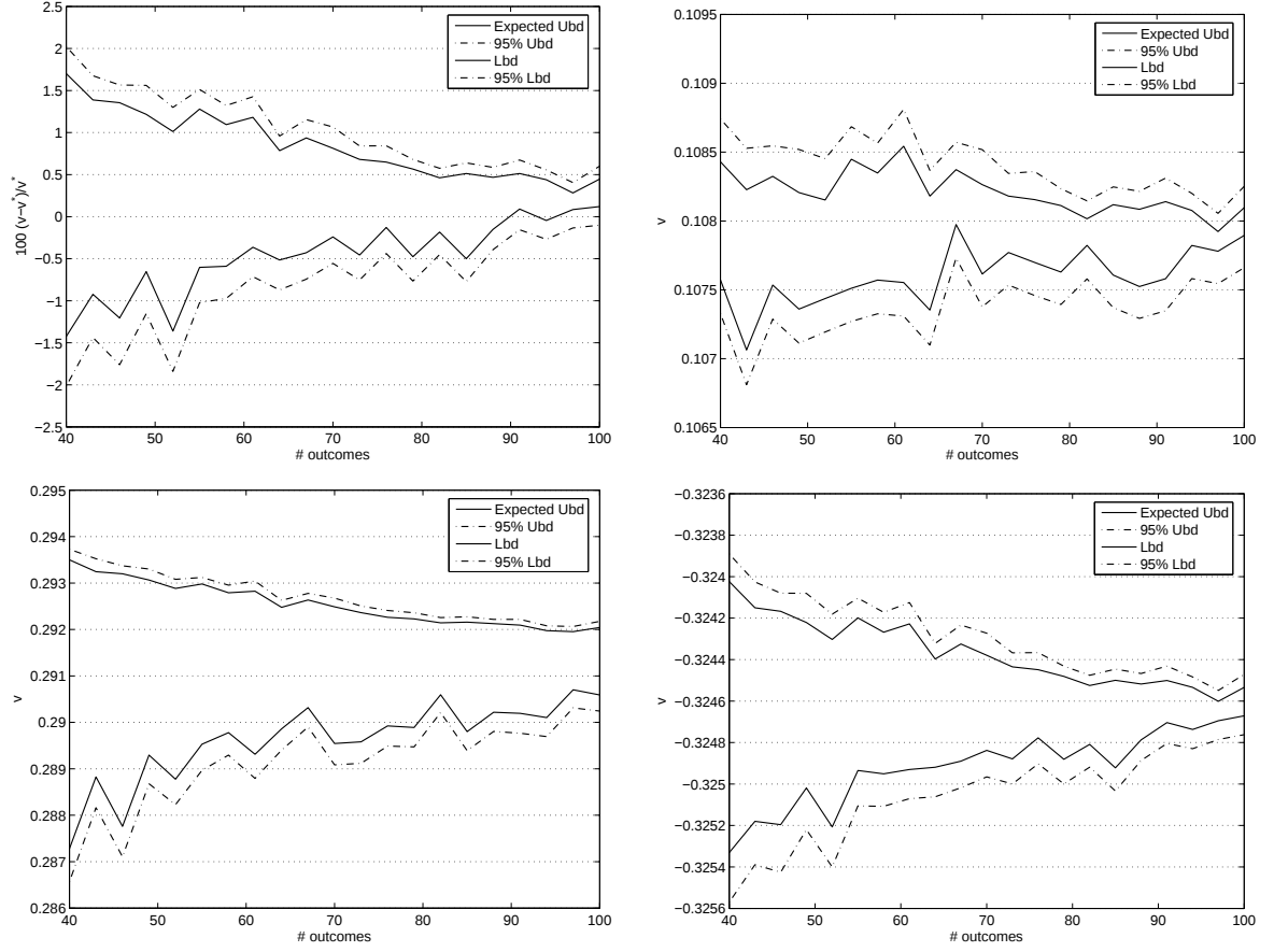
Figure 6: Objective function values for varying number of outcomes. Upper left: Scaled logarithmic utility function. Upper right: Logarithmic utility function with transaction costs. Lower left: Piecewise linear utility function. Lower right: Exponential utility function.
