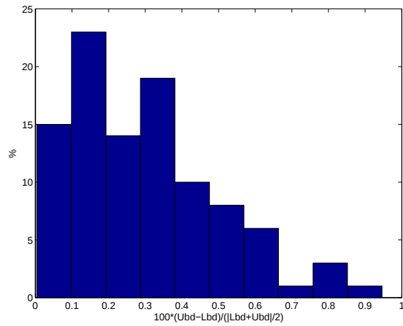
Figure 10: Histogram of gap for randomly generated \mu^a , \sigma^a , and c_{a_1 a_2} .
