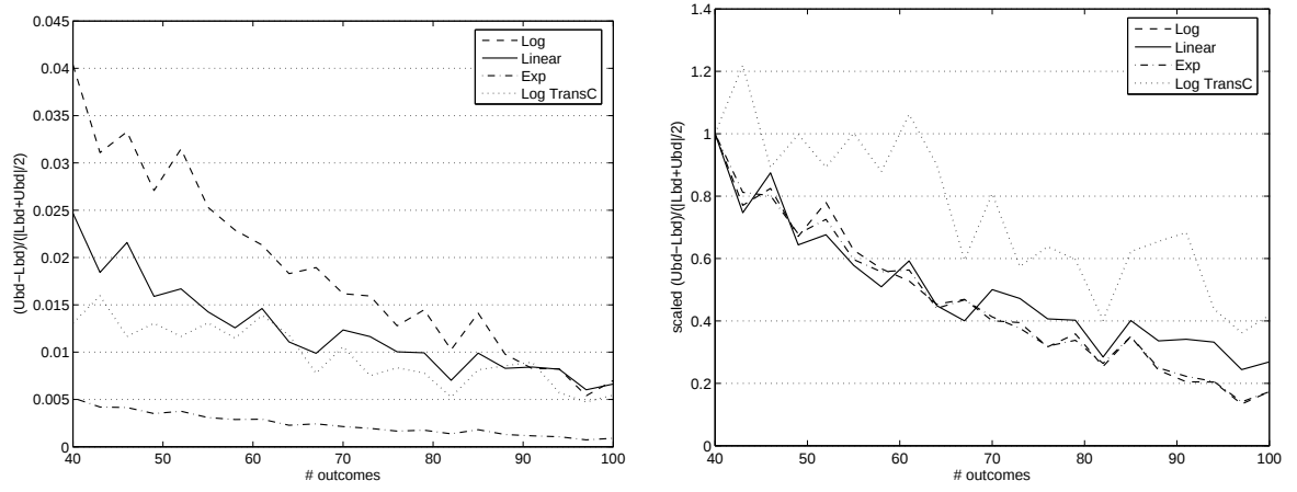
Figure 7: Left: Gap between 95% upper bound and 95% lower bound for varying number of outcomes. Right: Same as left but scaled.
