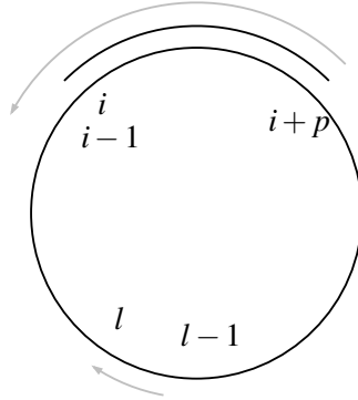
Figure 1: The incidence vector of a row of A consists of the nodes \{i, i+1, \dots, i+p\} which are consecutive on the cycle in clockwise order. Its corresponding arc in \mathcal{S}_L is the arc (i+p, i-1) . The arc (l-1, l) in \mathcal{T}_L corresponds to the lower bound x(l) \geq 0 .
