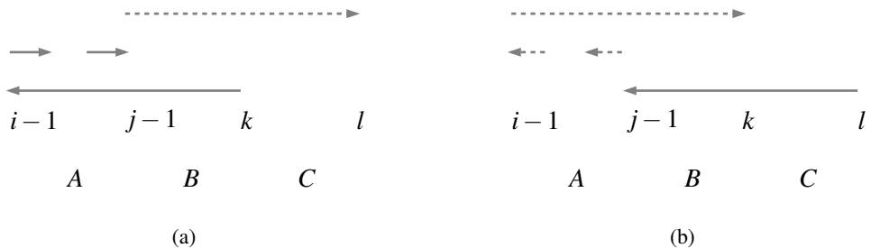
Figure 2: (a) depicts an arc (k, i-1) \in \mathcal{S}_L , followed by arcs in \mathcal{T}_L and the arc (j-1, l) \in \mathcal{S}_R . (b) depicts the situation, where the intermediate arcs are in \mathcal{T}_R .
