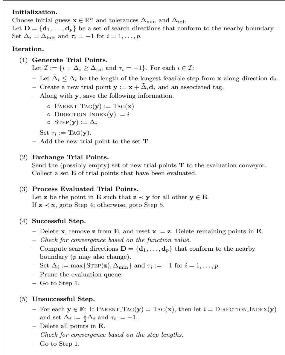
Fig. 1. APPS Algorithm
