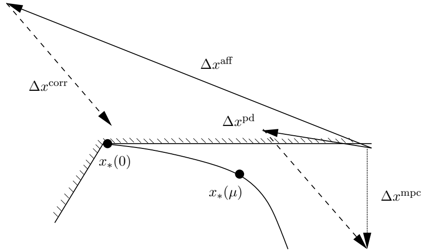
Figure 4: An unfavorable corrector step.
