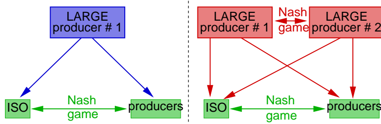
Figure 1: Structure of Stackelberg games and multi-leader multi-follower games
