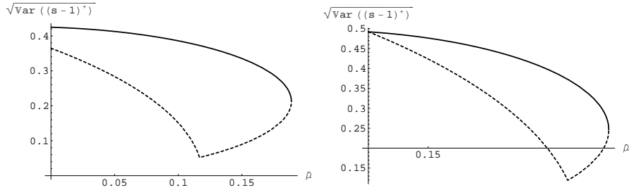
Figure 7: Upper and lower semiparametric bounds for the risk associated to a given expectation on the payoff of a European call option. Left: \underline{q}(\mu, \gamma, \hat{\mu}) (dashed) and \bar{q}(\mu, \gamma, \hat{\mu}) (solid) for \gamma = 1.2, \mu = 0.95 , as a function of \hat{\mu} . Right: \underline{q}(\mu, \gamma, \hat{\mu}) (dashed) and \bar{q}(\mu, \gamma, \hat{\mu}) (solid) for \gamma = 1.2, \mu = 1.1 , as a function of \hat{\mu} .
