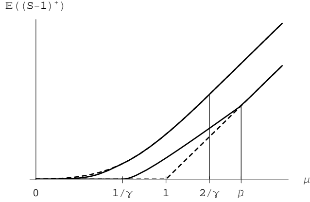
Figure 4: Third-order (solid lines) vs. second-order (dashed lines) semiparametric bounds for the payoff of a European call option when \beta \gg \gamma^2 (plots of \bar{p}(1, \mu, \gamma\mu^2) , \underline{p}(1, \mu, \gamma\mu^2) , \rho(\mu, \gamma, \beta)^+ , \underline{p}(1, \mu, \gamma\mu^2, \beta\mu^3) , generated with \gamma = 1.5 , and \beta = 3 , as a function of \mu ).
