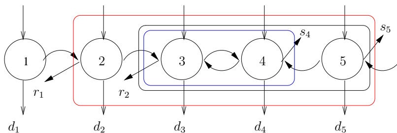
Figure 3: Coefficients of x_j , j \in S in inequality (8).
