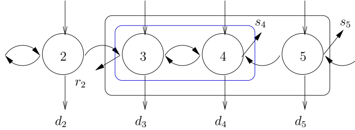
Figure 2: Coefficients of x_j , j \in S in inequality (7).
