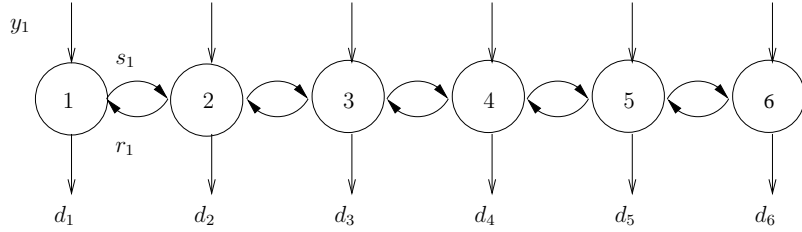
Figure 1: Fixed-charge network for lot-sizing with backlogging.
