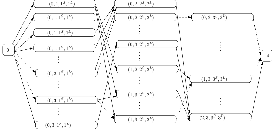
Figure 5: Graph G for separation for inequalities (53).
