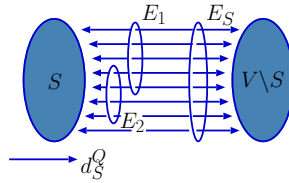
Figure 4: An undirected cutset with selected cut edges
