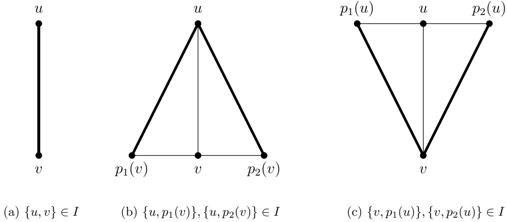
Figure 3: The three cases where e\{u, v\} is true. Edges which belong to the set I are drawn bold.
