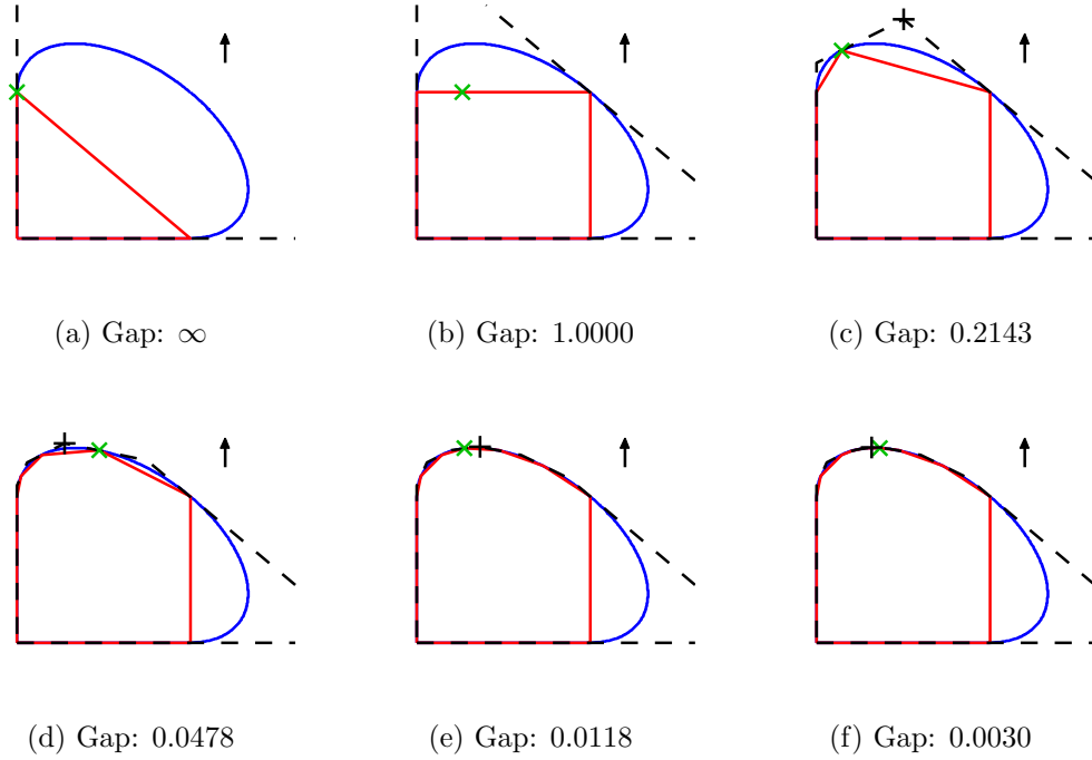
Figure 1: Iterations for Example 11
