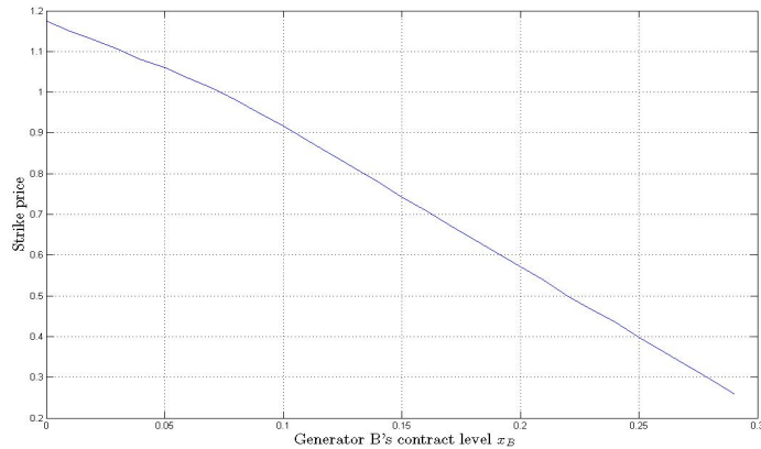
Figure 2: The strike price w.r.t. contract level x_B .
