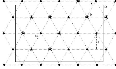
(b) Adjacent node sets for supernodes si and sj .
