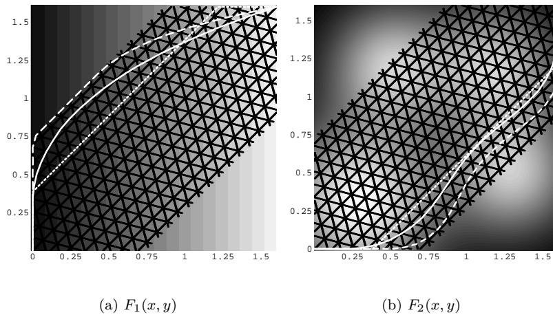
FIG. 5.1. Contour plot of functions F_1(x, y) and F_2(x, y) overlaid with the nodes of cellular network with parameters (i, j, M) = (24, 0, 24) . The lighter regions have higher function values. The shading scale on the two plots is not the same. Some parts of the region which are not length feasible have not been meshed. The edges are not shown to avoid cluttering the diagram. The paths corresponding to the upper bound in the cellular network are the solid white lines. The paths corresponding to the relaxed weight constraint \bar{L}(1 + \gamma) are the long dashed lines. Both problems were solved using the Gaussian scheme. We also calculated the upper bound paths given by a grid network of 721 by 721 nodes which are shown as the short dashed lines. We can see that the cellular network produces a smoother path than the grid network.
