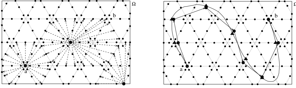
(a) Diagram of network showing how nodes (black dots) are placed and the leaving edges (dashed arrows) for selected nodes.
