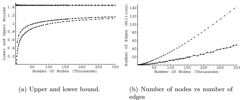
FIG. 5.2. The upper and lower bounds for the C-LCMCPP for the function F_1(x, y) vs the number of nodes. The squares are the lower bounds for i = M and the triangles are the results when i and M are optimised for an approximately constant number of nodes. The stars are the upper bounds for the i = M case and the diamonds are the upper bounds for the optimised i and M case. We can see that the optimisation offers a improvement on the lower bound. We can also see a diminishing return on the improvement to the lower bound as we use more nodes. The number of edges vs the number of nodes is also given in (b) in which the stars indicate the i = M case and the diamonds indicate the i and M optimised case.
