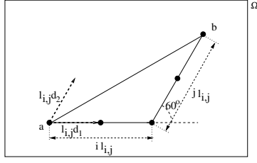
(a) Construction diagram for T(i, j) .
