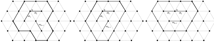
FIG. 4.3. Diagrams of the shapes of the regions around end node b .
