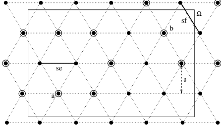
(c) Boundary supernode sets for superedges se and sf .
