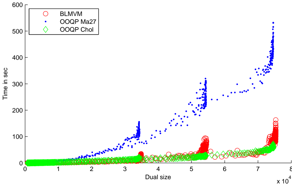
Figure 6. Execution time dependence on number of constraints.
