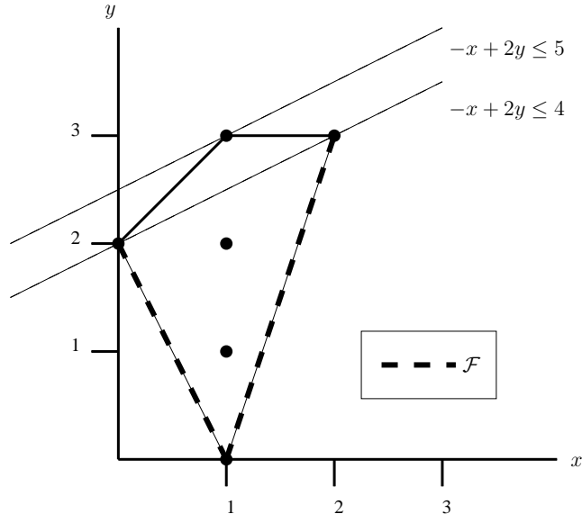
Figure 2: An example of the bilevel feasibility cut.
