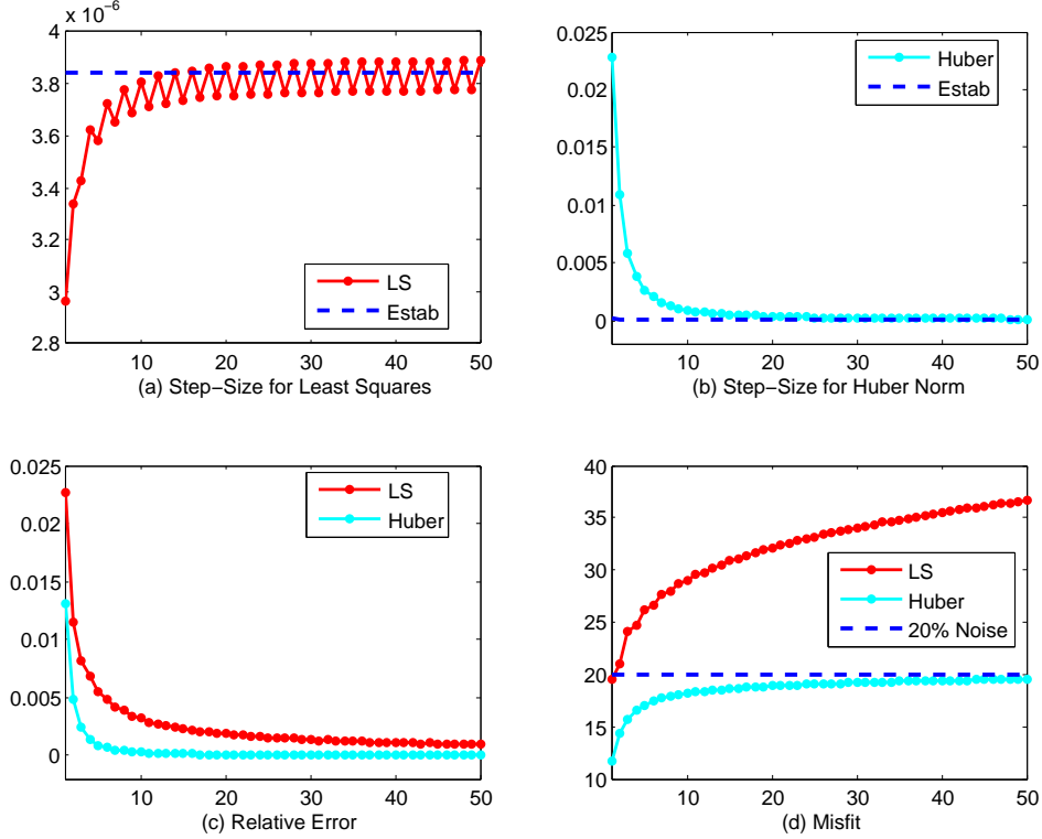
Figure 3: Discrete dynamics for the test problem Cameraman in Figure 4(a) with 20% white noise added. Two regularizations, LS ( \gamma large) and Huber switching ( \gamma by (18)), are compared.
