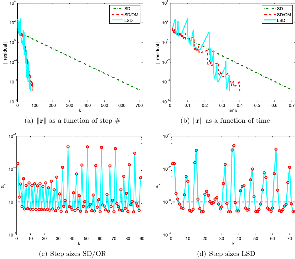
Figure 2: Residual norms and step size sequences on a log scale for the Poisson problem of Examples 1 and 2 with m = 225 .
