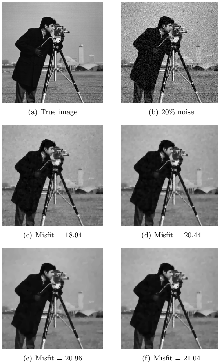
Figure 4: Using Algorithm (19) with adaptive \gamma by (18). (a) Clean image Cameraman ; (b) image corrupted by 20% Gaussian white noise; (c) denoised image using SD step size (20a) for error tolerance tol = 10^{-4} on \hat{e}_k of (21a): iters = 21, \eta_{21} = 18.94 ; (d) denoised image using LSD step size (20b) for the same tol : iters = 14, \eta_{14} = 20.44 ; (e) same as (c) with tol = 10^{-5} : iters = 382, \eta_{382} = 20.96 ; (f) same as (d) with tol = 10^{-5} : iters = 117, \eta_{117} = 21.04 . The CPU time is roughly proportional to the number of steps required.
