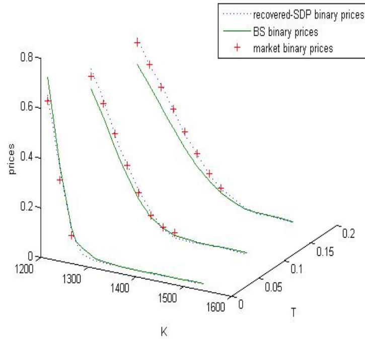
Figure 9: Recovered binary call prices from S&P500 data using the SDP approach against Black-Scholes binary prices and S&P500 2008 binary prices.
