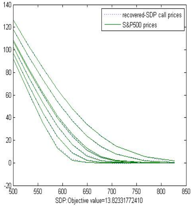
Figure 6: Recovered expected prices plotted against the S&P500 1995 prices for the seven maturities (QP and SDP approaches).
