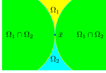
FIGURE 10. \theta[\Omega_1, \dots, \Omega_n](\bar{x}) = \infty
