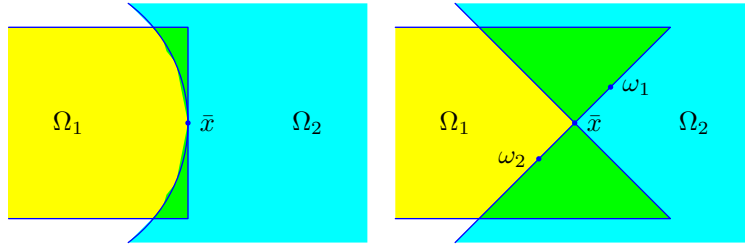
FIGURE 8. Stationarity and approximate stationarity
