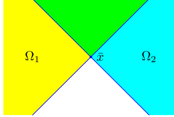
FIGURE 9. Regularity
