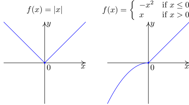
FIGURE 2. Inf-stationarity
