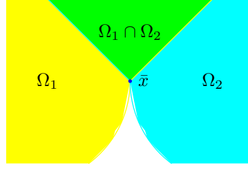
FIGURE 11. (R)_S holds while (MI)_S does not
