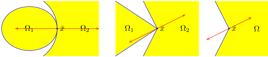
FIGURE 7. Nonconvex separation property
