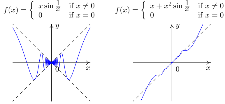
FIGURE 3. Approximate inf-stationarity
