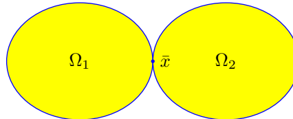
FIGURE 4. Extremality of two convex sets
