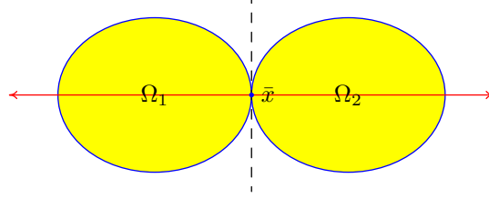
FIGURE 6. Separation property
