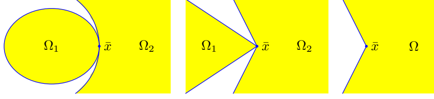
FIGURE 5. Extremal collections of sets
