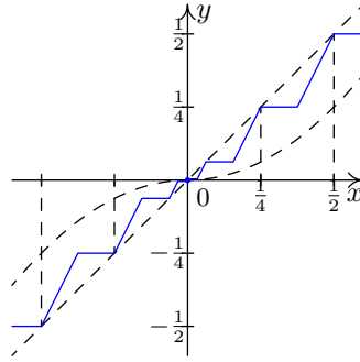
FIGURE 13. Example 3
