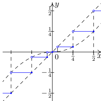
FIGURE 12. Example 2
