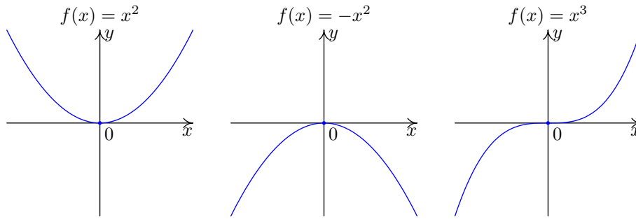
FIGURE 1. Stationarity: differentiable case
