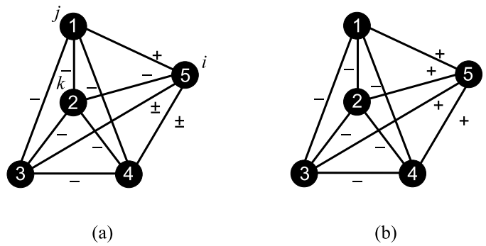
Figure 3: Consider the negative clique K = \{1, 2, 3, 4\} . (a) Conditions in Theorem 4.8 guarantee the existence of vertices j, k such that \{i, j, k\} does not define an odd negative cycle. (b) For any choice of vertices j, k \in K there is an odd negative cycle C = \{i, j, k\} .
