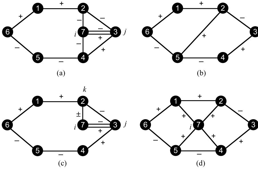
Figure 2: Consider C = \{1, 2, 3, 4, 5, 6\} . (a) The odd negative cycle C induces a facet-defining inequality of P_{G,s} . For vertex i = 7 , the choice of j = 3 makes condition (iii) satisfied. (b) The odd negative cycle C is a composition of cycles C' = \{2, 3, 4, 5\} and C'' = \{5, 6, 1, 2\} where C'' \in C^o(E) . The odd negative cycle inequality written to C'' defines a facet of P_{G,s} . (c) Since (2, 7), (3, 7) \in E^- \cap E^+ , y(C) = 5 implies y_7 = 0 . (d) The graph induced by C \cup \{7\} contains more than two odd negative cycles; y(C) = 5 implies y_7 = 0 .
