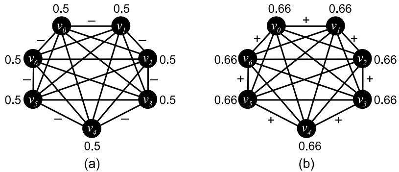
Figure 6: Fractional solutions to the LP relaxation of formulation Y(G, s) cutted off by cycle (a) negative and (b) positive clique inequalities.
