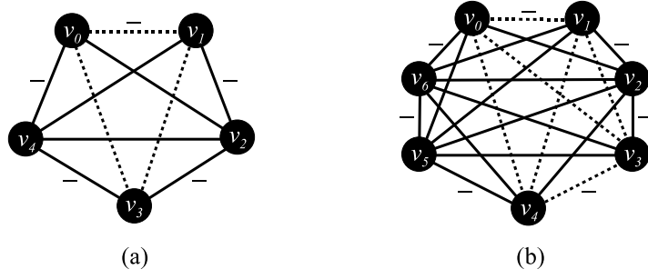
Figure 4: Cycle negative odd cliques with |K| = 5 and |K| = 7 . Signs of positive edges are omitted. Dotted edges define (a) an odd negative cycle when t = 0 and (b) a partitionable clique when t = 0 ; both of them used in the proof of Theorem 4.11.
