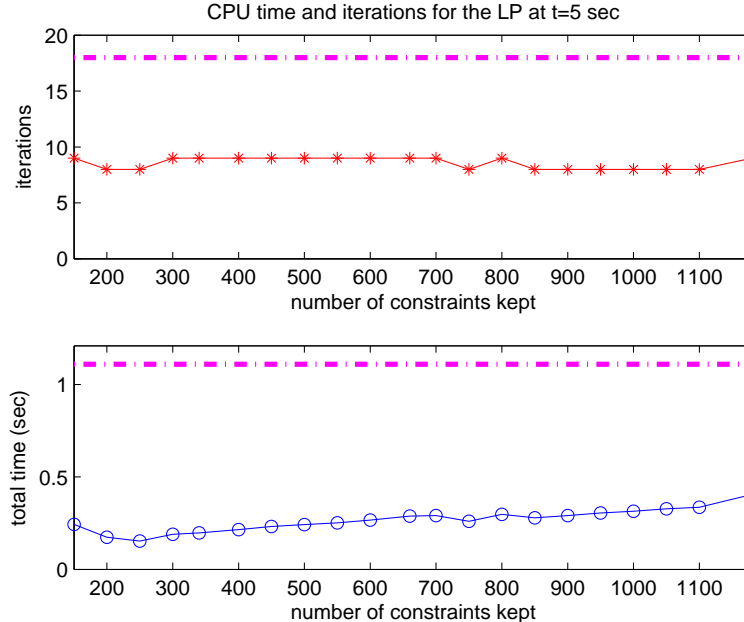
Figure 5: CPU time and iteration of solving the problem at 5 sec by IrMPC with varying number |Q| of kept constraints; see (blue) circles and (red) stars. MPC takes much longer to solve this problem; see the dashed (magenta) line.
