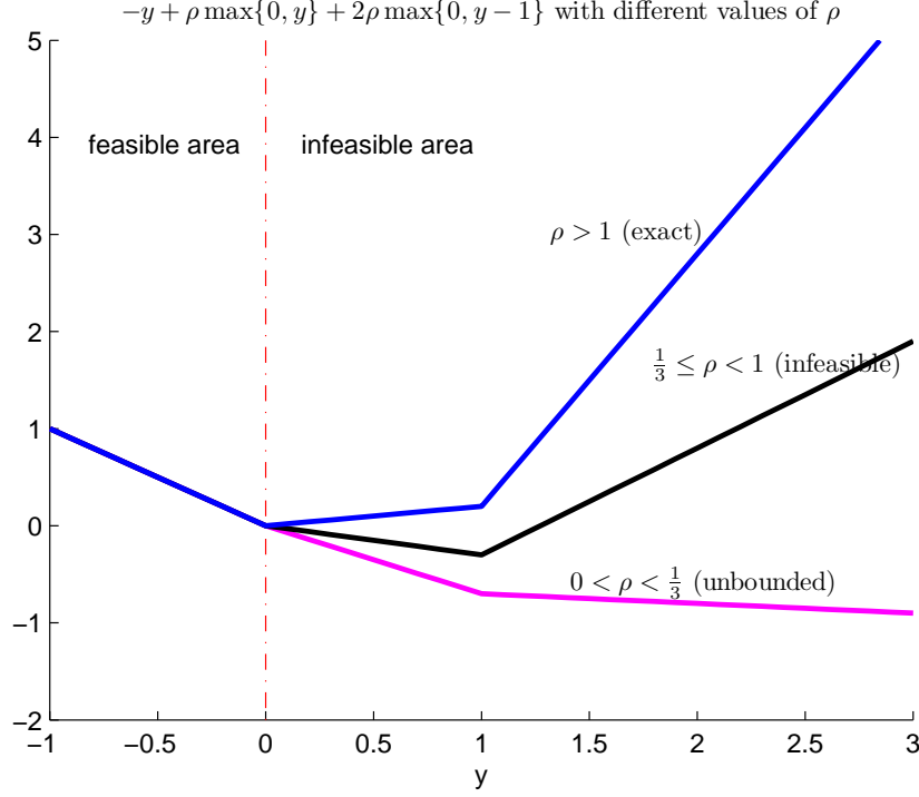
Figure 1: The objective function of problem (11) is displayed with different penalty parameter values. When \rho < \frac{1}{3} , problem (11) is unbounded. When \rho \in [\frac{1}{3}, 1) , it is bounded but the minimizer y_*^\rho = 1 is infeasible for (10). When \rho > \rho_* = 1 , y_*^\rho = 0 solves (10) as desired.
