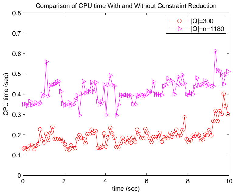
Figure 4: CPU time in seconds by IrMPC to solve the 10 sec RHC process with |Q| \approx 300 and |Q| = n = 1180 (corresponding to the case with unreduced constraints). For the former, in 58 cases, |Q| was increased slightly above 300 due to A^Q losing rank, as per Step 2 (iii) of Iteration IrPDIP.
