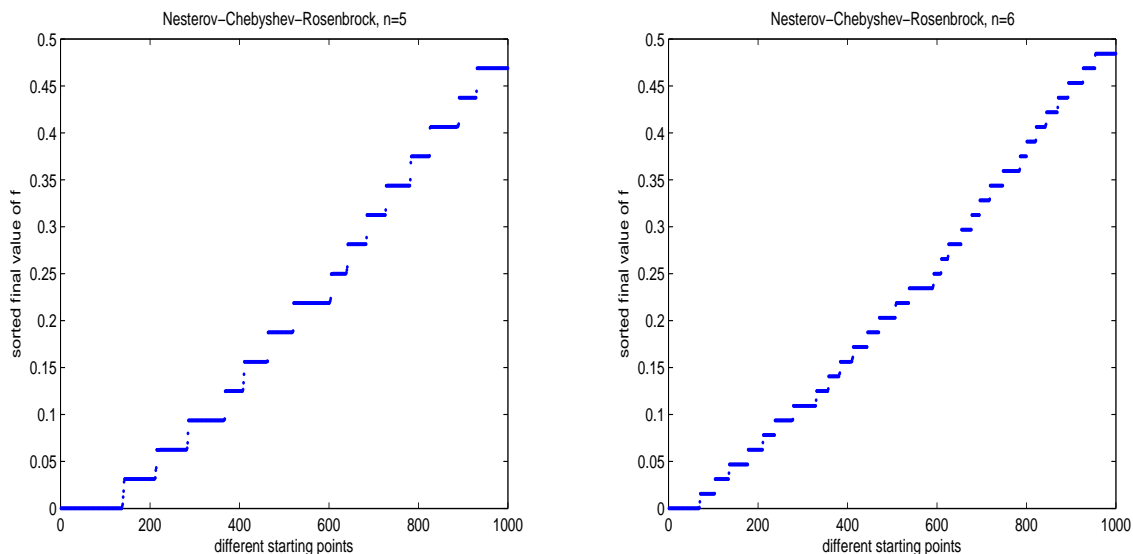
Figure 2: Left: sorted final values of f for 1000 randomly generated starting points, when n = 5 : BFGS finds all 16 Clarke stationary points. Right: same with n = 6 : BFGS finds all 32 Clarke stationary points.
