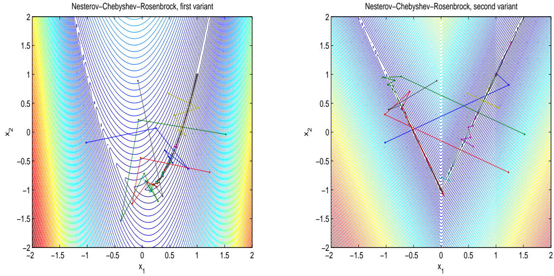
Figure 1: Contour plots for Nesterov’s first (left) and second (right) nonsmooth Chebyshev-Rosenbrock functions \hat{f} and f respectively, with n = 2 . Points connected by line segments show the iterates generated by the BFGS method (see Section 3) initialized at 7 different randomly generated starting points. For the first variant \hat{f} , convergence always takes place to the only Clarke stationary point: the global minimizer x^* = [1, 1]^T . For the second variant f , some runs of BFGS generate iterates that approximate the nonminimizing Clarke stationary point [0, -1]^T while others converge to the minimizer [1, 1]^T .
