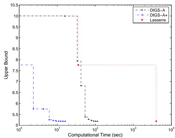
Fig. 2: Bounds comparison for Example 2.
