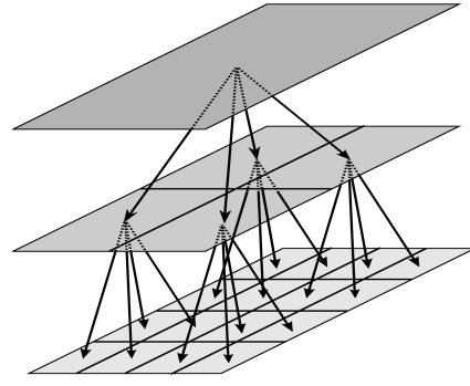
(a) Information structure of the aggregate model
