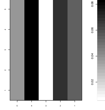
(b) Equilibrium density of the aggregated Markov Chain
