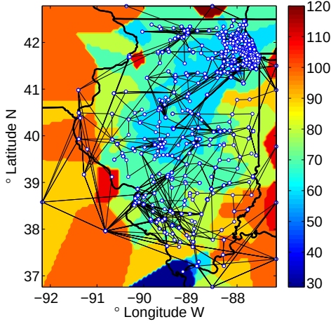
Fig. 1: Spatial field of locational marginal prices ($/MWh) under time-averaged conditions in Illinois grid.
