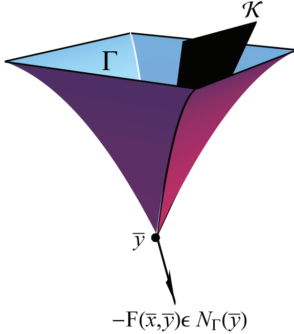
Figure 1: Illustration of the feasible set \Gamma defined by (23) and of the critical cone \mathcal{K} .
