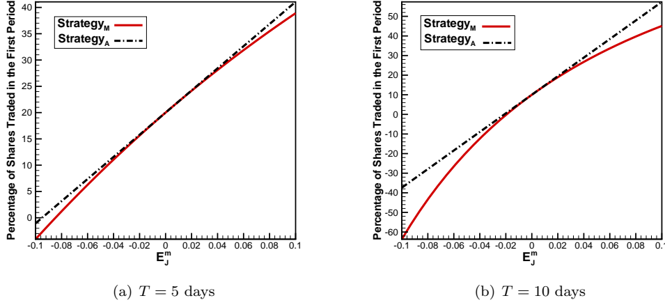
Figure 3: Comparison of the optimal execution n_1^* under the multiplicative jump model and under the additive jump model. Initial holding is \bar{S} = 10^7 shares. The total volatility is \sigma_{tot} = 0.03 .
