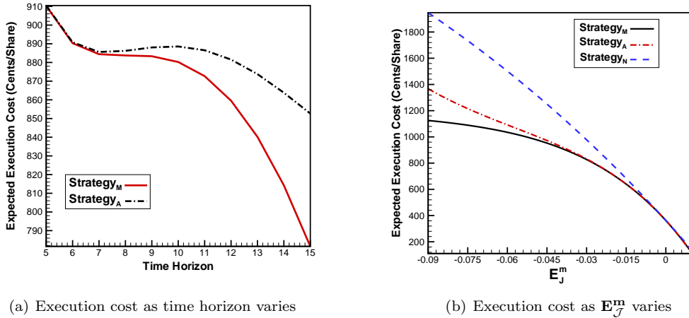
Figure 5: Comparison in the expected execution cost (cents per share). The expected costs in the plot were computed using Theorem 3.3 for Strategy M and Proposition D.1 for Strategy A . Initial holding is \bar{S} = 10^7 shares. The values specified for the model parameters yield \Sigma^m = 9.045 \times 10^{-3} . For Subplot (a), \lambda_x = 3.8, \mu_x^m = 9.901 \times 10^{-3}, \sigma_x^m = 9.901 \times 10^{-3}, \lambda_y = 0.2, \mu_y^m = 1.186 \times 10^{-2}, \sigma_y^m = 1.198 \times 10^{-2}, E_J^m = -3.560 \times 10^{-2}, \text{Cov}_J^m = 8.182 \times 10^{-4}
