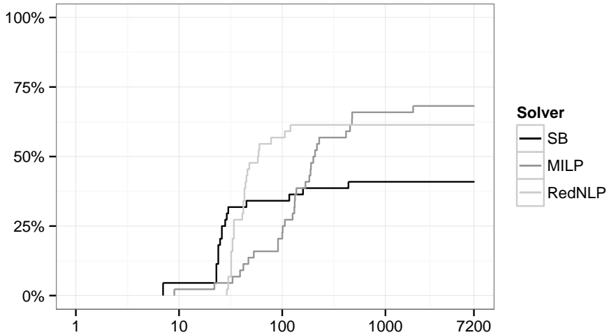
FIGURE 16. Profile of the run times (s) for test set AB6 including NLP validation; y -axis: percentage of confirmed or infeasible instances (total: 44)
