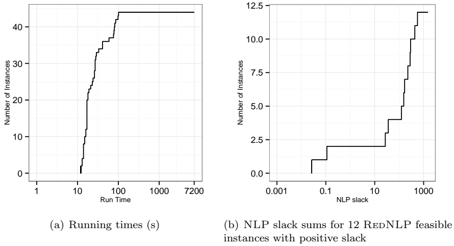
FIGURE 12. Numerical results on the second test set (AB6) for the REDNLP approach
