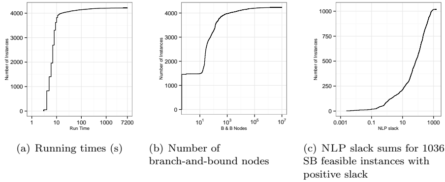
FIGURE 9. Numerical results on the first test set (SN4) for the SB approach
