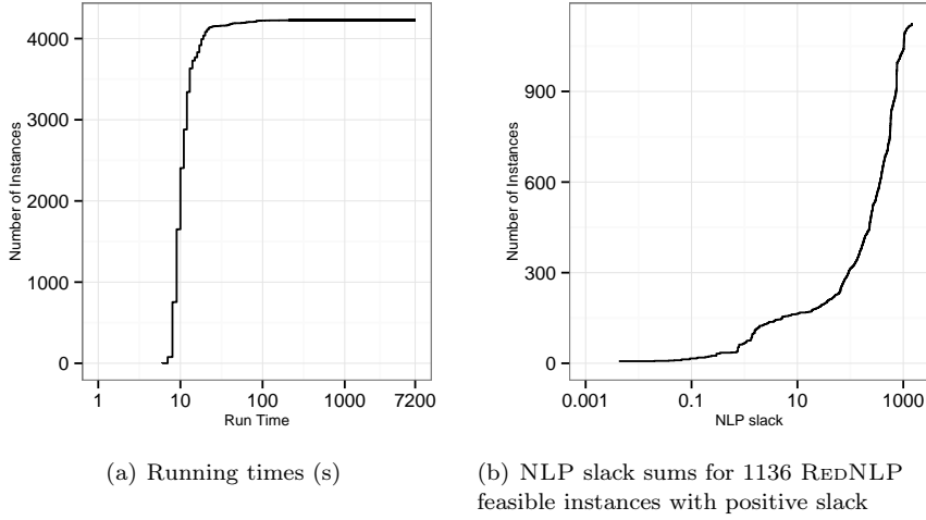
FIGURE 11. Numerical results on the first test set (SN4) for the REDNLP approach
