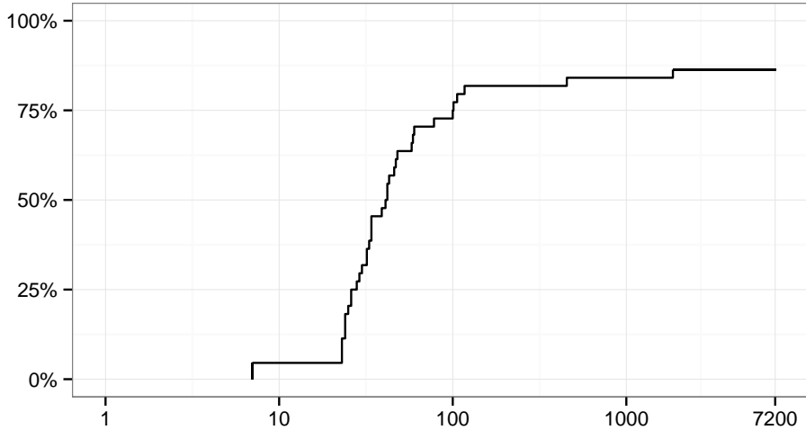
FIGURE 18. Profile of the run times (s) for the combined approach on test set AB6 including NLP validation; y -axis: percentage of confirmed or infeasible instances (total: 44)
