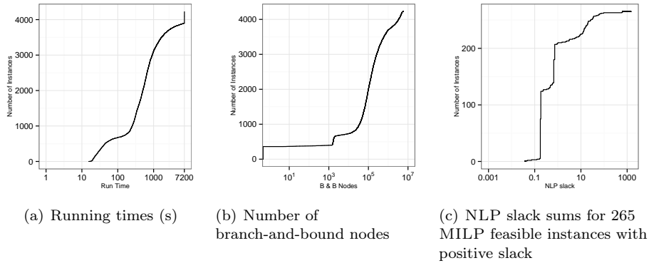
FIGURE 7. Numerical results on the first test set (SN4) for the MILP approach
