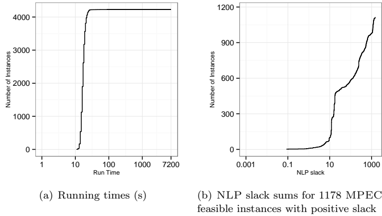
FIGURE 13. Numerical results on the second test set (SN4) for the MPEC approach
