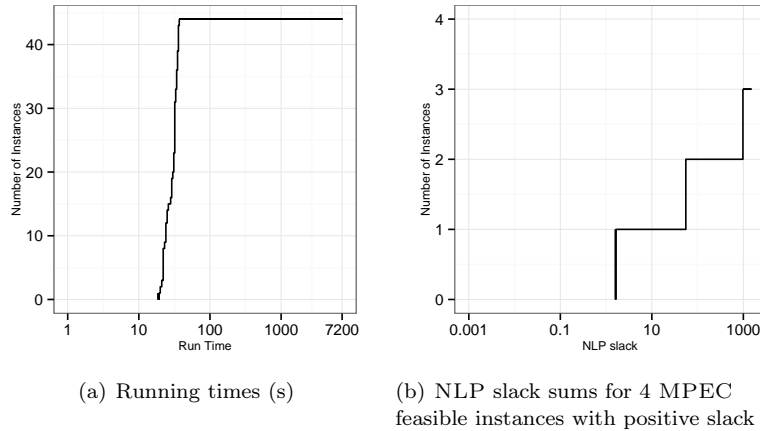
FIGURE 14. Numerical results on the second test set (AB6) for the MPEC approach
