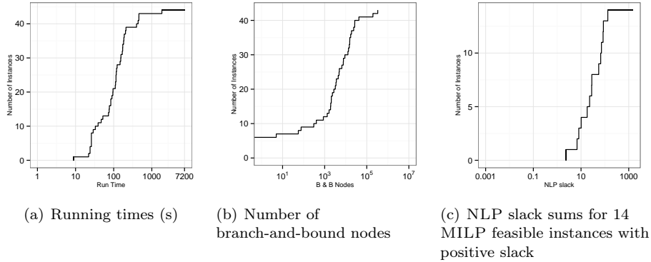
FIGURE 8. Numerical results on the second test set (AB6) for the MILP approach
