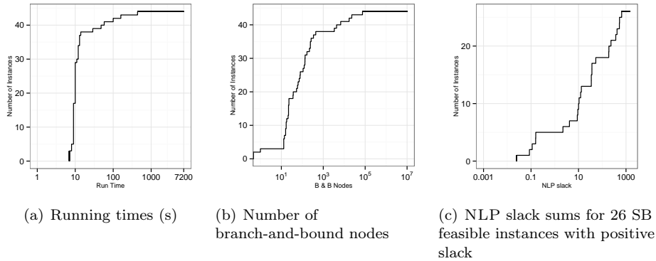
FIGURE 10. Numerical results on the second test set (AB6) for the SB approach
