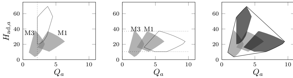
FIGURE 4. Resulting operation ranges for different combinations of two machines, M1 and M3: serial compression (first M3 then M1) (left); parallel compression (middle), and convex hull of all feasible points (right)
