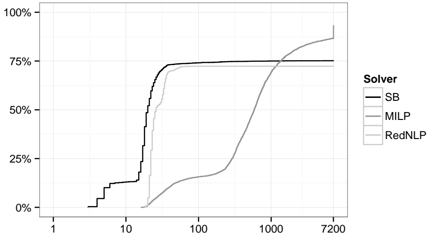
FIGURE 15. Profile of the run times (s) for test set SN4 including NLP validation; y -axis: percentage of confirmed or infeasible instances (total: 4227)
