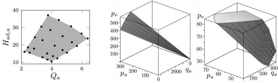
FIGURE 3. From the characteristic diagram of a compressor (left) over the (unbounded) cone (middle) to the operation range polytope (right)
