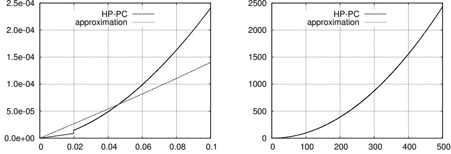
FIGURE 5. Discontinuous friction model \lambda^{\text{HPPC}} and its smooth approximation \phi for small flow rates (left) and large flow rates (right)
