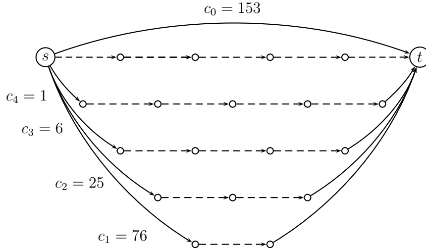
Figure 3: An instance associated with a disjoint paths graph in which all potential arcs need to be built in an optimal solution.
