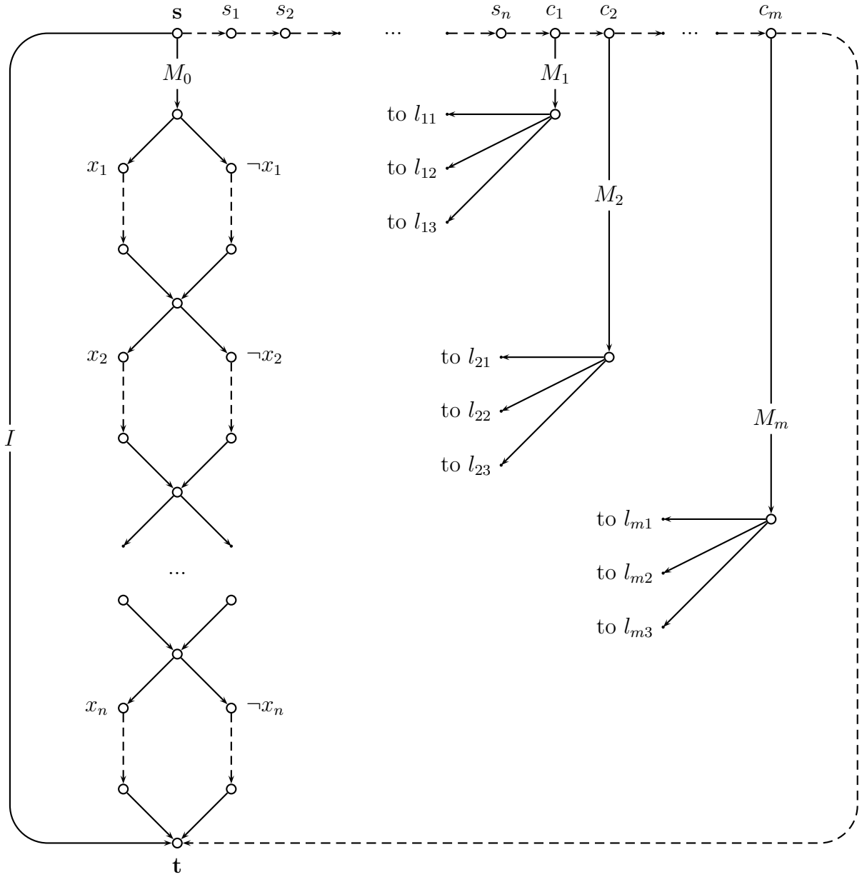
Figure 2: Instance of INDP-SP used in the reduction from 3-SAT.
