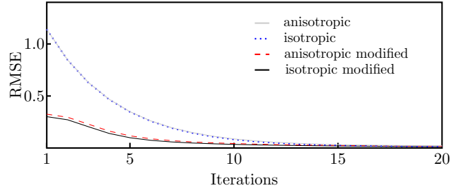
Figure 3: RMSE curves for image denoising: the case of white Gaussian noise with standard deviation \sigma = 0.12
