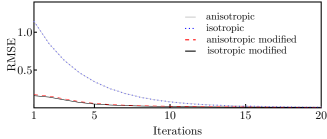
Figure 2: RMSE curves for image denoising: the case of white Gaussian noise with standard deviation \sigma = 0.06
