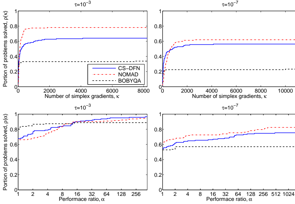
FIG. 3. Data (top) and performance (bottom) profiles for the 142 bound-constrained problems. Comparison among CS-DFN, NOMAD and BOBYQA
