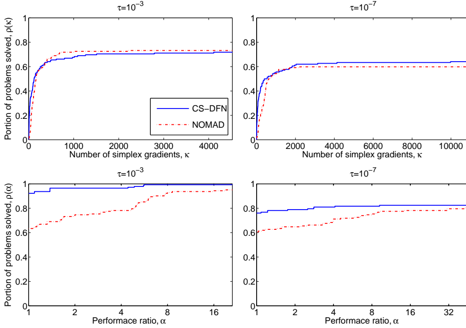
FIG. 5. Data (top) and performance (bottom) profiles for the 142 bound-constrained problems. Comparison among CS-DFN and NOMAD (without quadratic local models)
