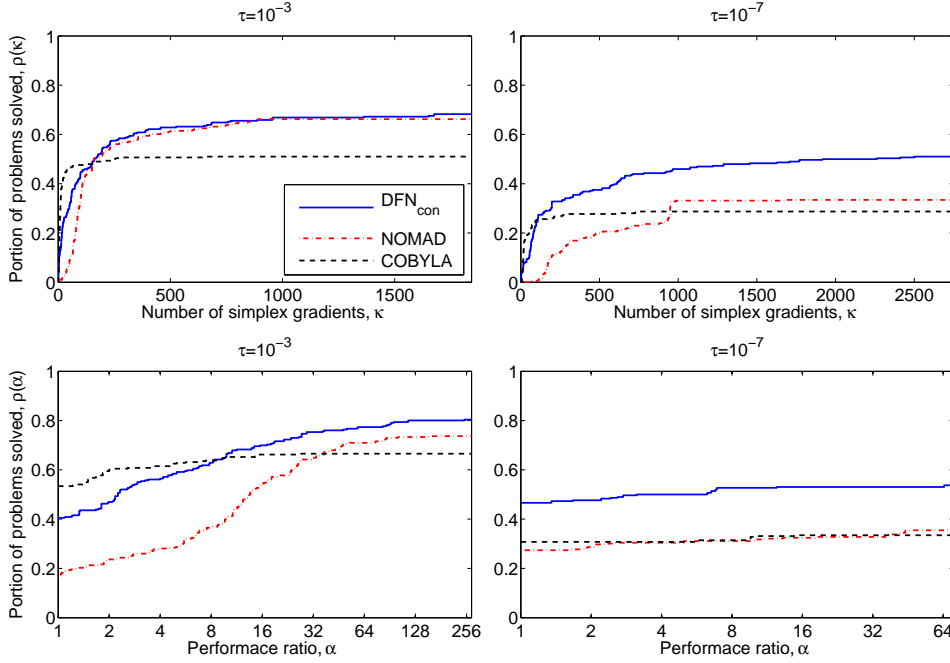
FIG. 9. Data (top) and performance (bottom) profiles for the 296 constrained problems. Comparison among DFN_{con} , NOMAD (without quadratic models) and COBYLA
