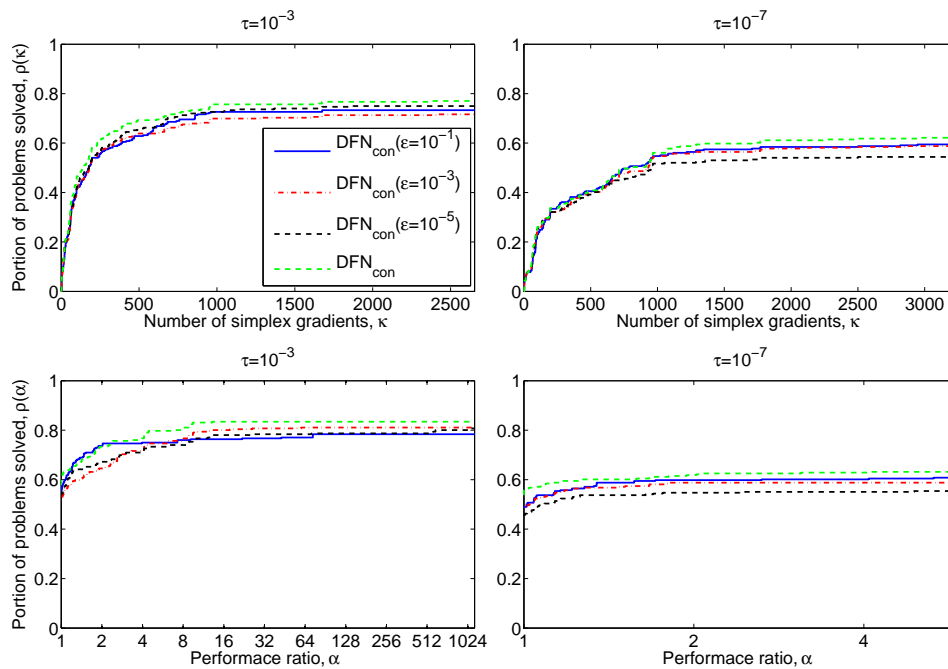
FIG. 6. Data (top) and performance (bottom) profiles for the 296 constrained problems. Comparison among different versions of DFN_{con} with different strategies for updating the penalty parameter \varepsilon
