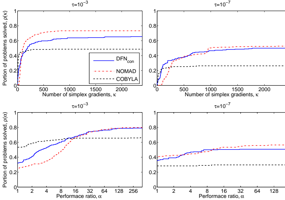
FIG. 7. Data (top) and performance (bottom) profiles for the 296 constrained problems. Comparison among DFN_{con} , NOMAD and COBYLA
