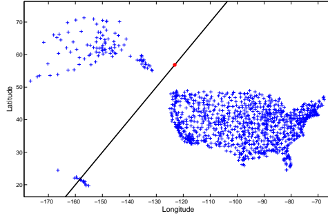
Figure 3: A Generalized Fermat-Torricelli Problem with US Cities
