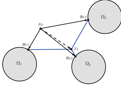
Figure 1: MM Algorithm for a Generalized Fermat-Torricelli Problem
