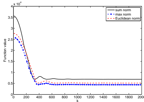
Figure 2: Generalized Fermat-Torricelli problems with different norms
