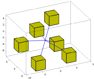
Figure 4: A generalized Fermat-Torricelli problem with MM method
