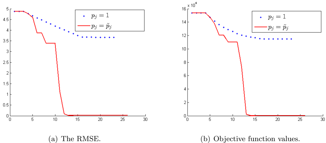
Figure 3: Results of one run of Algorithm 7.1 when using probabilities p_j = 1 (dotted line) and p_j = \tilde{p}_j (solid line).
