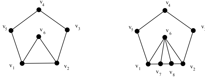
FIGURE 3. The graph G' is obtained from G after the clique subdivision of edge v_1v_2 .
