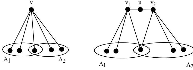
FIGURE 2. A 1-stretching operation on node v .
