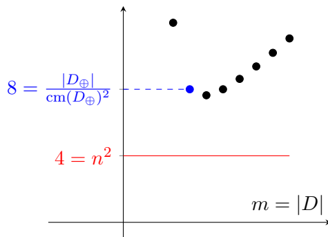
Figure 1: Illustration of inequality (8) in \mathbb{R}^2 for PSSs making uniform adjacent angles. The plot depicts the values of |D|/\text{cm}(D)^2 for |D| = 3, 4, \dots, 10 .
