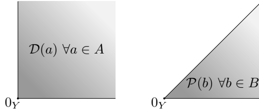
Figure 1: Illustration of the concepts of Definition 2.4.
