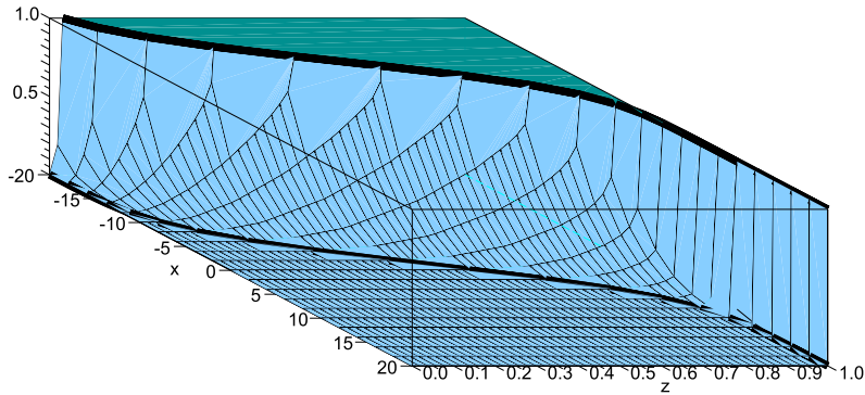
Figure 2: Value function (at time 0).
