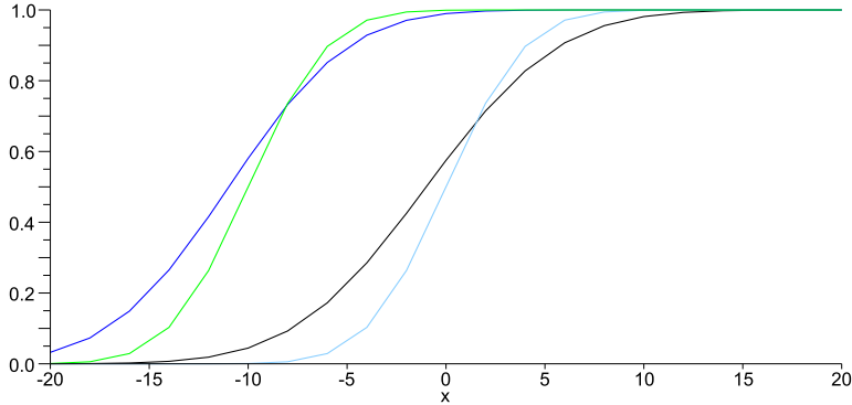
Figure 1: Boundaries (at time 0).
