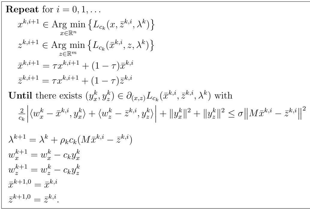
Figure 3: The DQA-RE algorithm.
