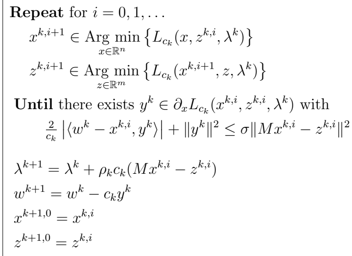
Figure 2: The GS-RE algorithm.
