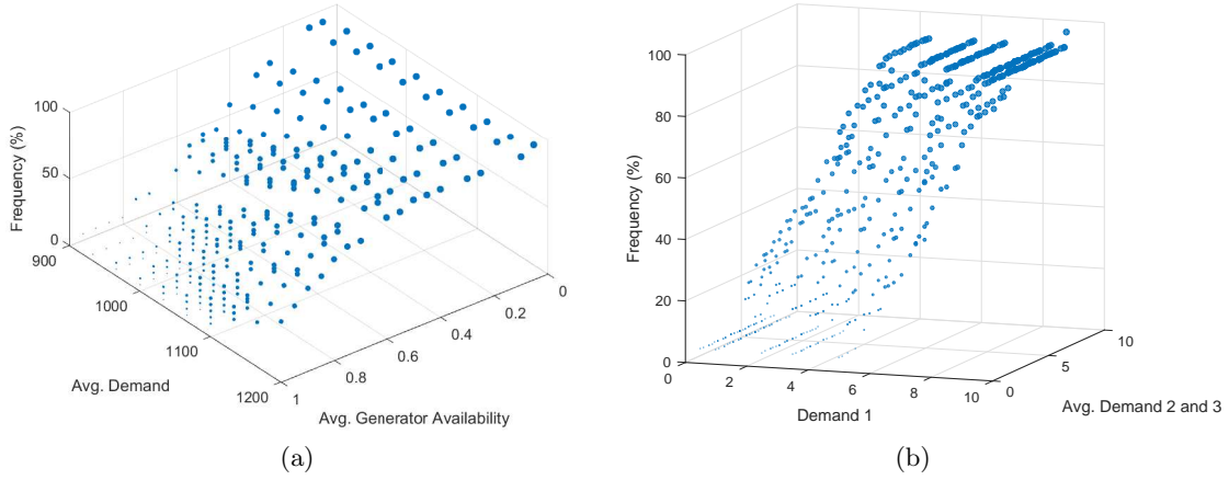
Figure 1: The percentage of cases a scenario is effective for APL1P.
