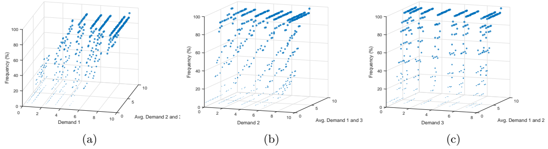
Figure 2: The percentage of cases a scenario is effective for PGP2.
