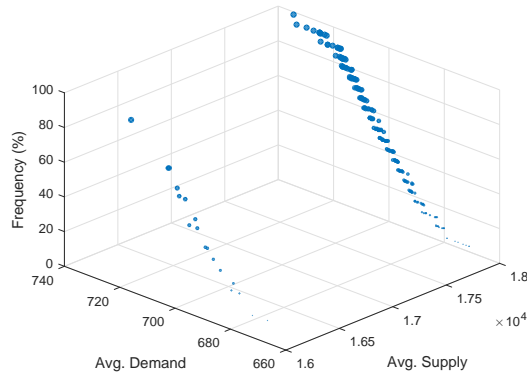
Figure 3: The percentage of cases a scenario is effective for Water Allocation problem across different levels of robustness. The two distinct portions in the graph correspond to a drought in the Colorado River (low avg. supply) and no drought in the Colorado River (high avg. supply).
