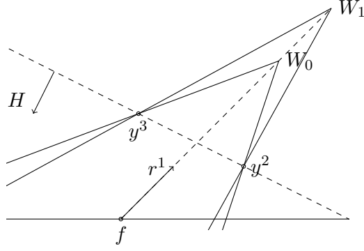
Figure 6: Wedges W_0 and W_1 in the configuration of Lemma 14.
