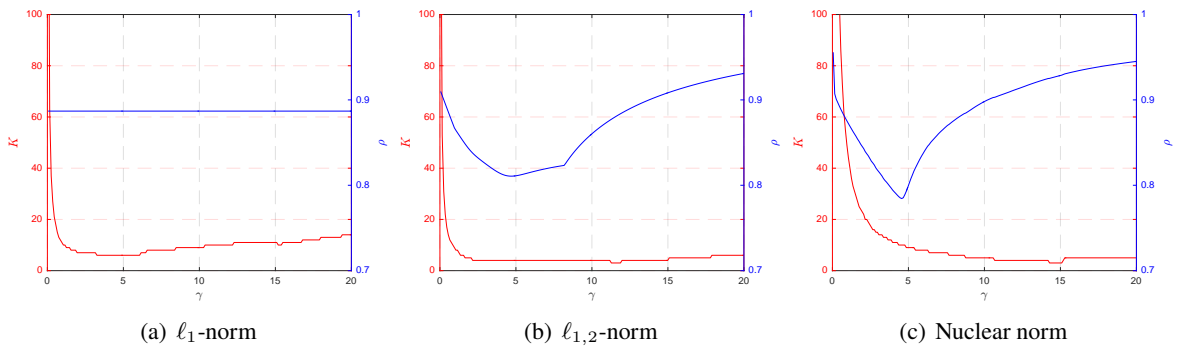
Figure 4: Number of iterations ( K ) needed for identification and local linear convergence rate ( \rho ) as a function of \gamma when solving problem (9.1) with different functions J in Table 1. (a) \ell_1 -norm. (b) \ell_{1,2} -norm. (c) Nuclear norm.
