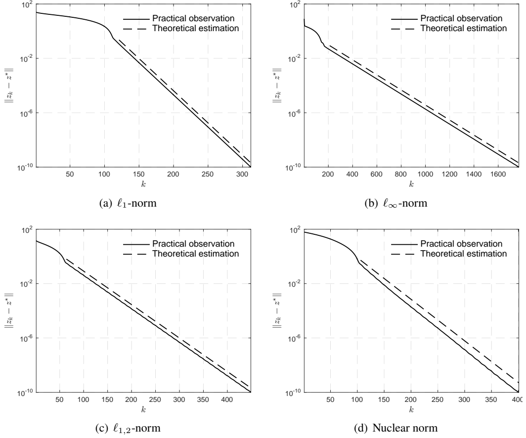
Figure 1: Observed (solid) and predicted (dashed) convergence profiles of DR (1.1) in terms of \|z_k - z^*\| . (a) \ell_1 -norm. (b) \ell_\infty -norm. (c) \ell_{1,2} -norm. (d) Nuclear norm. The starting point of the dashed line is the iteration at which the active manifold of J is identified.
