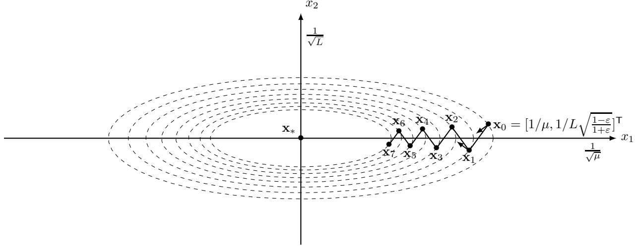
Figure 2: Illustration Example 5.2 for n = 2 and \varepsilon = 0.3 (small arrows indicate direction of negative gradient).
