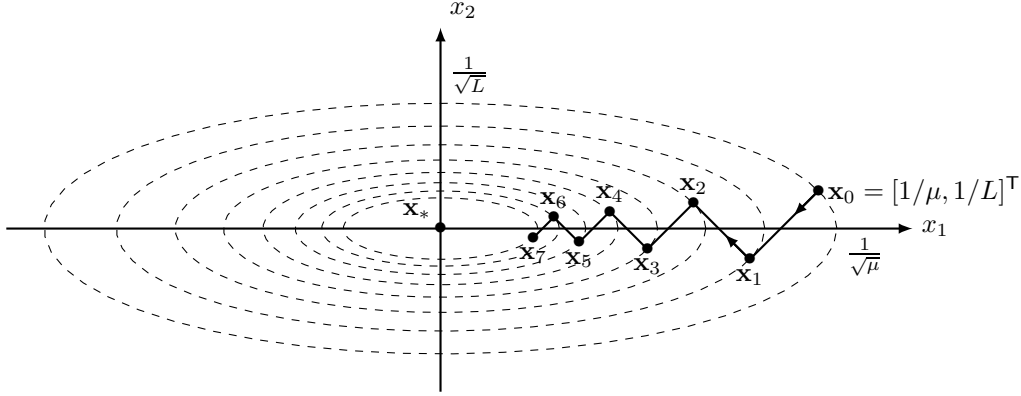
Figure 1: Illustration of Example 1.3 for the case n = 2 (small arrows indicate direction of negative gradient).
