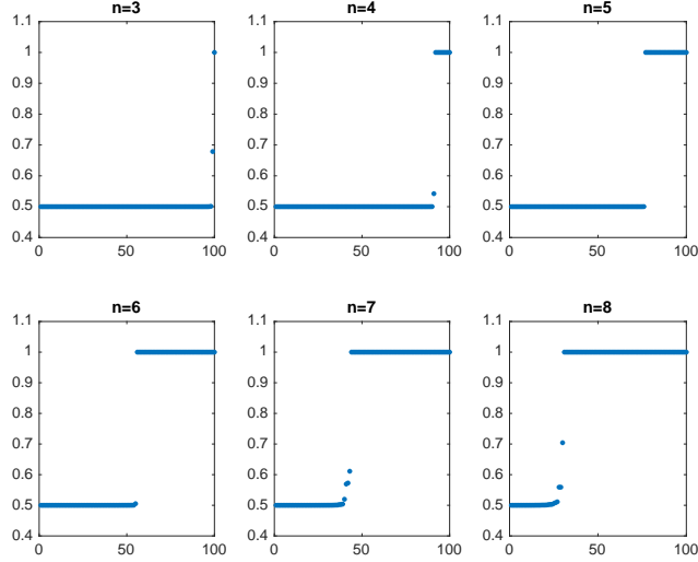
Figure 2: Results for minimizing f over c and A for n = 3, \dots, 8 . Each panel shows the final values of f obtained in 100 runs of BFGS from normally distributed starting points, sorted into ascending order.
