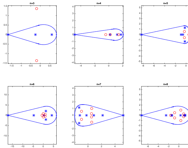
Figure 4: “Ice Cream Cone” stationary points of the Crouzeix ratio f , discovered while minimizing f for n = 3, \dots, 8 . The panel for each n shows the boundary of W(A) (solid blue), the eigenvalues of A (blue asterisks) and the roots of p (red circles), where p and A are respectively the final polynomial and matrix corresponding to the final value of f that is closest to one , all plotted in the complex plane.
