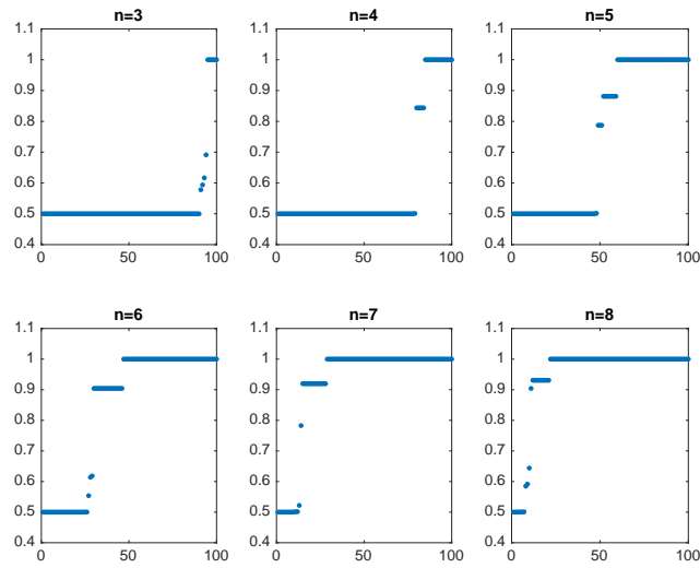
Figure 5: Results for minimizing f over A for n = 3, \dots, 8 , with p fixed to the monomial \zeta^{n-1} . Each panel shows the final values of f obtained in 100 runs of BFGS from normally distributed starting points, sorted into ascending order.
