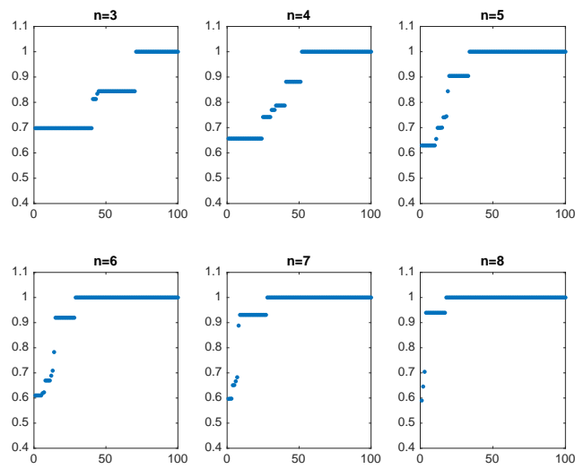
Figure 7: Results for minimizing f over A for n = 3, \dots, 8 , with p fixed to the monomial \zeta^n . Each panel shows the final values of f obtained in 100 runs of BFGS from normally distributed starting points, sorted into ascending order.
