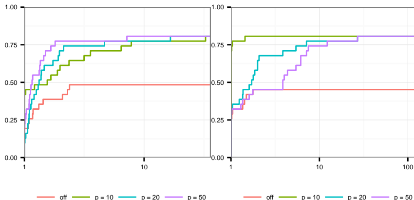
FIGURE 6. Log-scaled performance profiles of the rounding heuristic applied every p \in \{10, 20, 50\} branch-and-bound nodes within the MIQP approach with symmetry breaking constraints of Méndez-Díaz and Zabala and deactivated root node heuristic; cf. Sect. 4.2.2. Left: running times. Right: Node count
