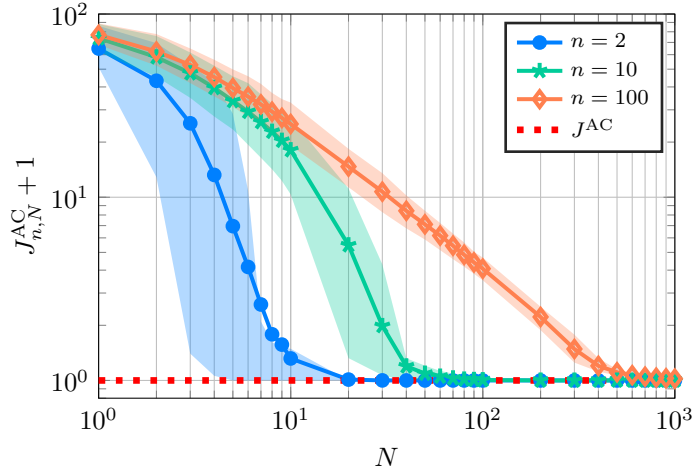
FIGURE 4. The objective performance J_{n,N}^{\text{AC}} is computed using (18) for Example 7.2. The red dotted line is the optimal value approximated by n = 10^3 and N = 10^6 , which amounts to 0 as also reported in [42].
