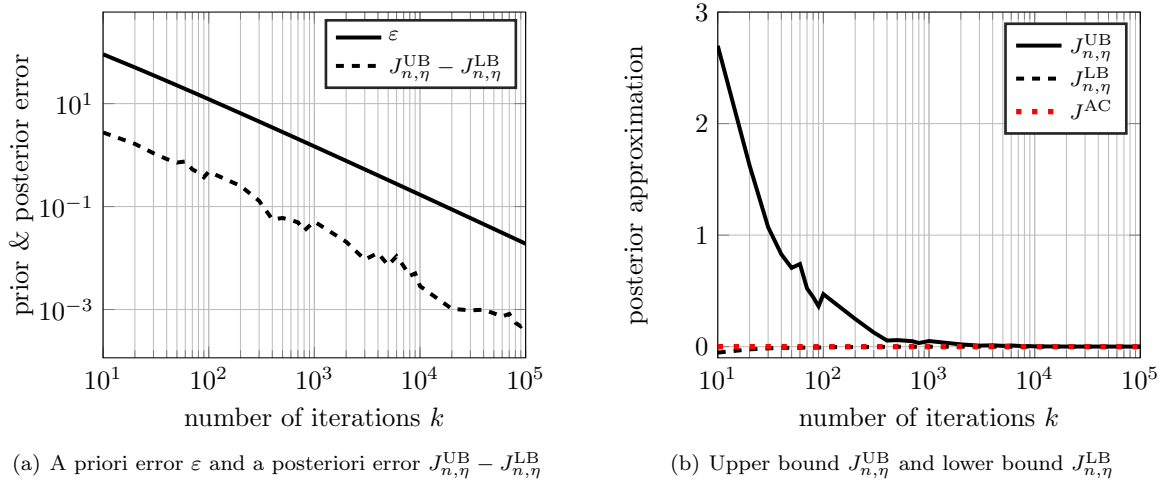
FIGURE 5. The results and error bounds are obtained by Algorithm 1 with n = 10 for Example 7.2. The red dotted line is the optimal solution computed as indicated in Figure 4.
