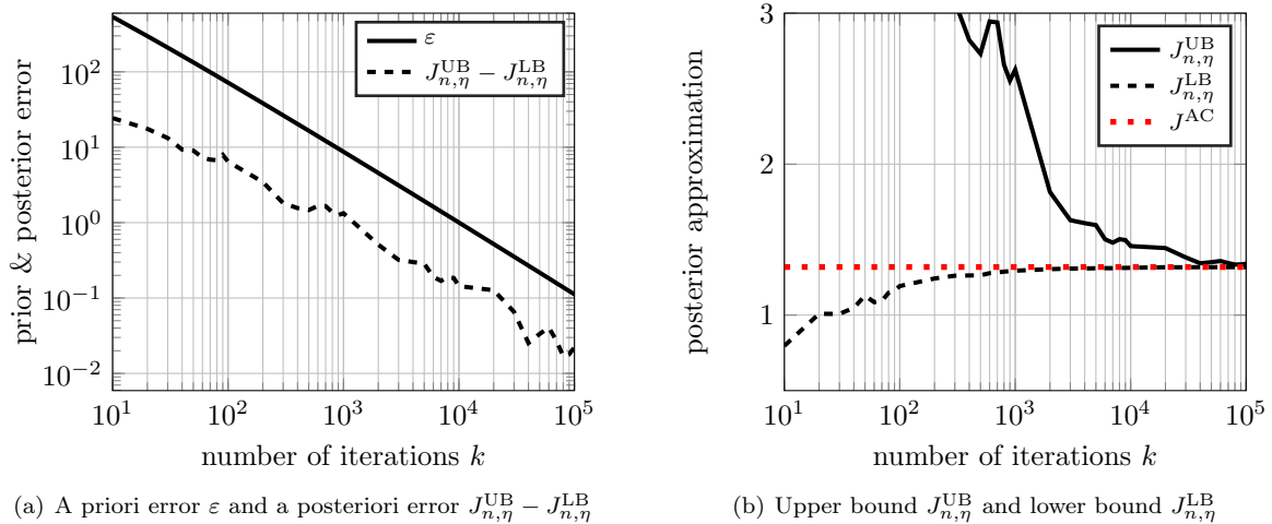
FIGURE 3. The results and error bounds are obtained by Algorithm 1 with n = 10 for Example 7.1. The red dotted line is the optimal solution computed as indicated in Figure 2.
