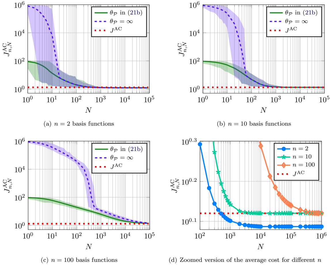
FIGURE 2. The objective performance J_{n,N}^{AC} is computed using (18) for Example 7.1. The red dotted line denoted by J^{AC} is the optimal solution approximated by n = 10^3 and N = 10^6 .
