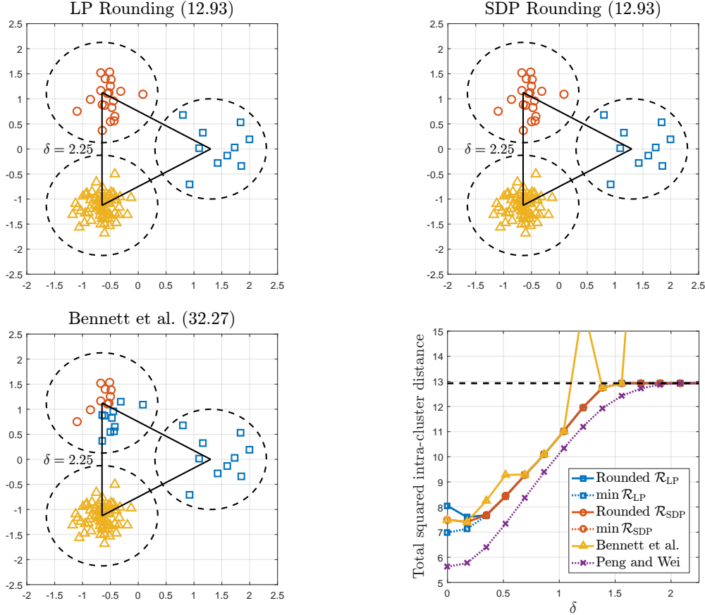
Figure 3 Comparison between different algorithms for (cardinality-constrained) K -means clustering for 100 datapoints where the cardinalities are given by (n_1, n_2, n_3) = (10, 20, 70) . Indicated in parentheses next to the panel titles are the respectively achieved sums of squared intra-cluster distances.
