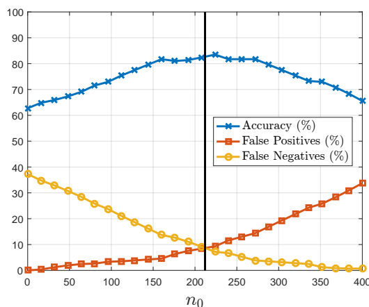
Figure 4 Outlier detection for breast cancer diagnosis.
