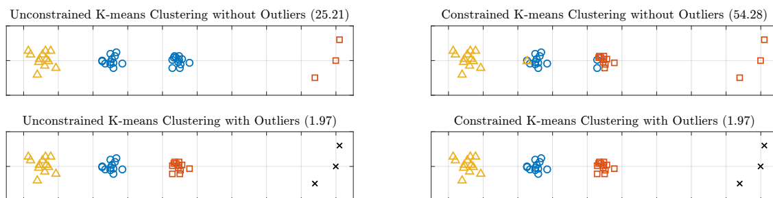
Figure 1 Sensitivity of the (un)constrained K -means clustering problem to outliers. Indicated in parentheses next to the panel titles are the respectively achieved sums of squared intra-cluster distances.
