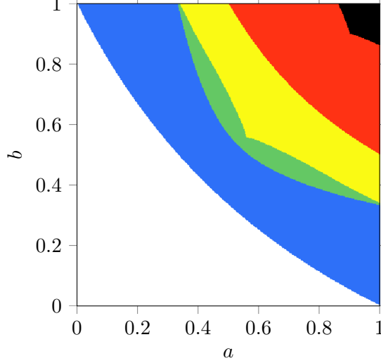
Figure 1: The colored region corresponds to \text{rank}_+(S(a, b)) = 4 . The top right region (black) corresponds to \xi_{1,+}^+(S(a, b)) > 3 , the two top right regions (black and red) together correspond to \tau_+^{\text{sos}}(S(a, b)) > 3 , the three top right regions (black, red and yellow) to \xi_{2,+}^+(S(a, b)) > 3 , and the four top right regions (black, red, yellow, and green) to \xi_{3,+}^+(S(a, b)) > 3
